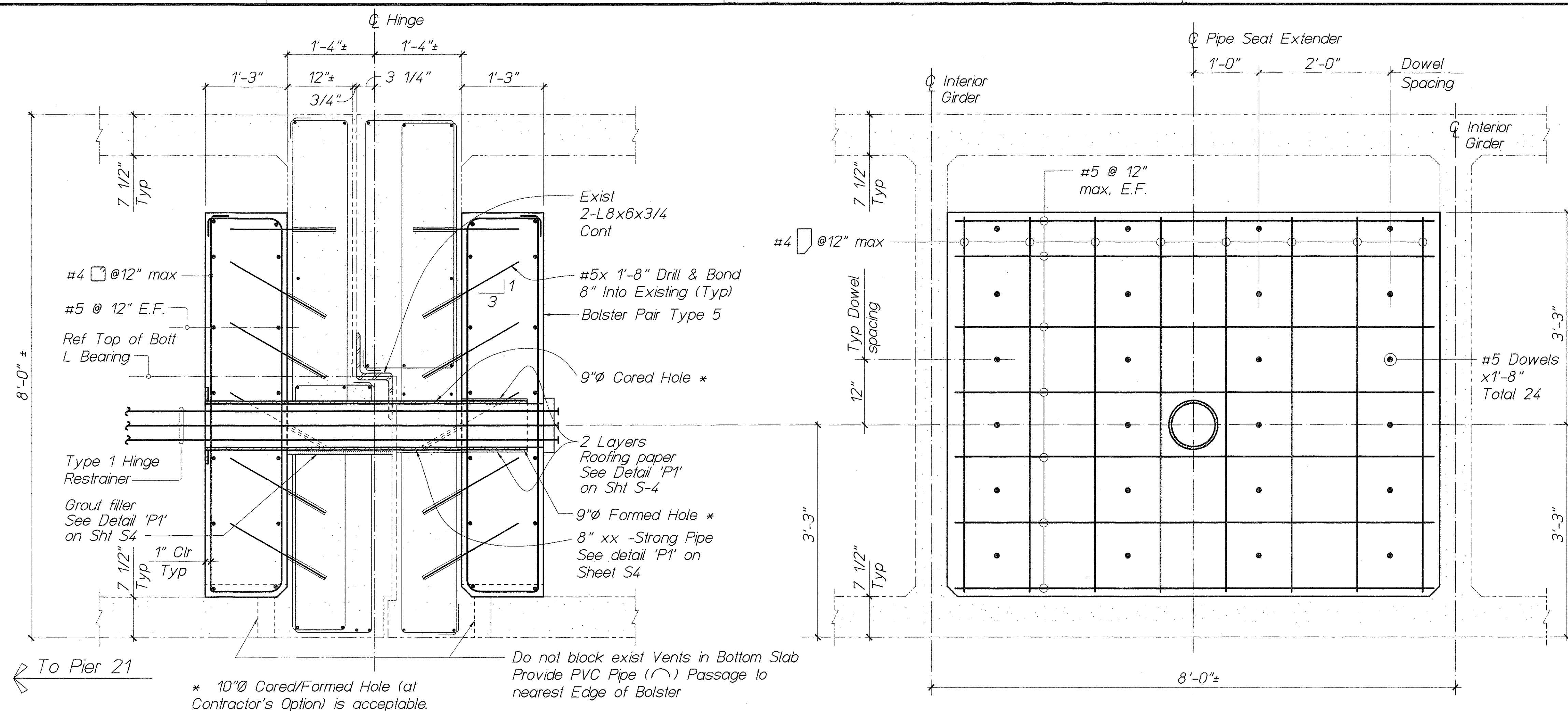
HINGE DETAIL 1 - SECTION 1"=1'-0"
