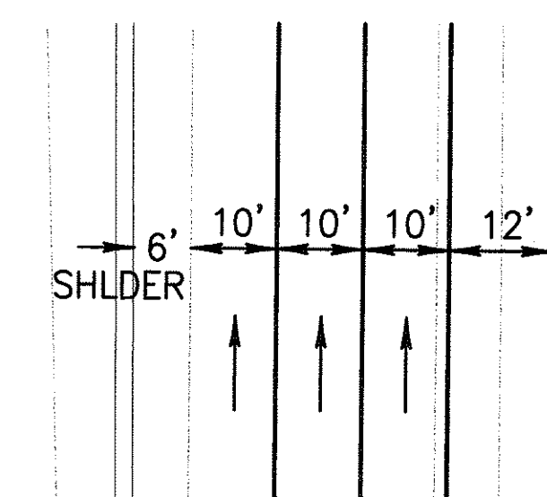
TYPICAL SECTION "B-B" TEMPORARY LANE SHIFT SCALE: 1"=20'
