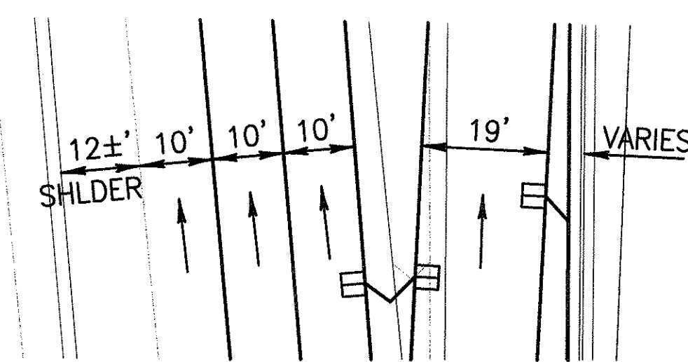
TYPICAL SECTION "A-A" TEMPORARY LANE SHIFT SCALE: 1"=20'
