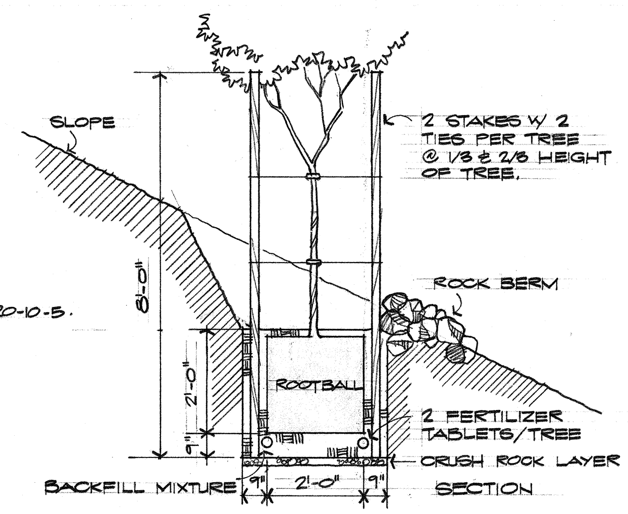
TYP. TREE PLANTING DETAIL NO SCALE
