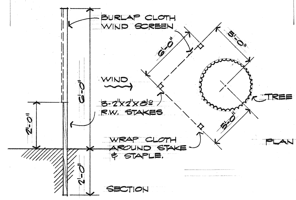
TYP. WIND SCREEN DETAIL NO SCALE
