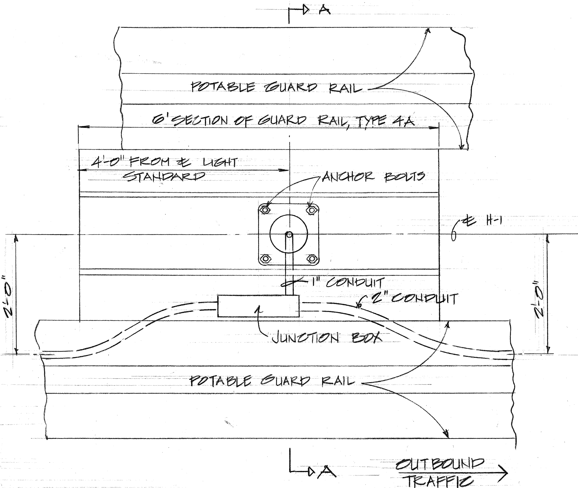
1.2 TYPICAL PLAN E-2 SCALE: 1"=1'-0"
