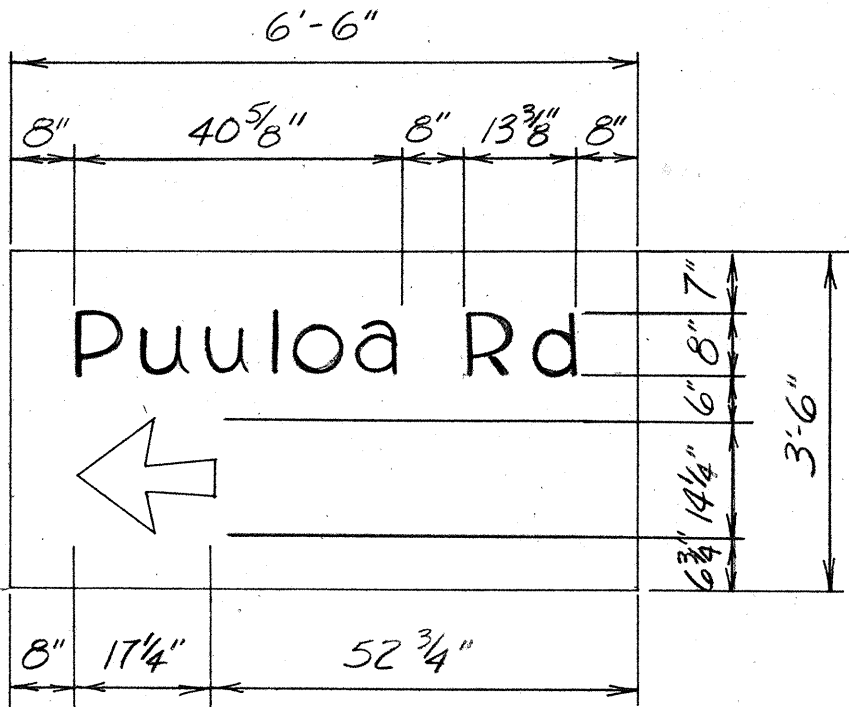
SIGN D-13
