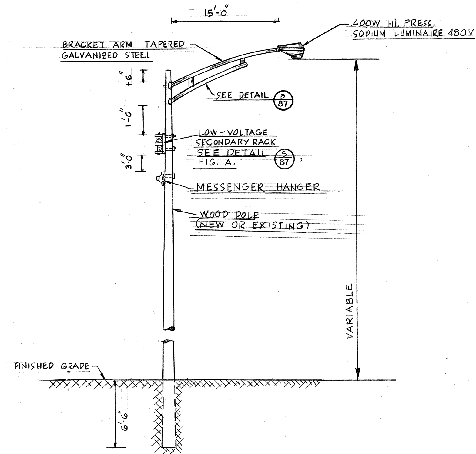
WOOD POLE DETAIL (1/87) NTS.
