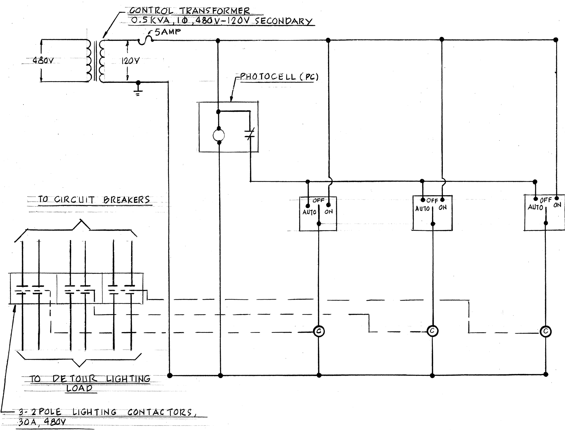
LIGHTING CONTROL WIRING DIAGRAM
