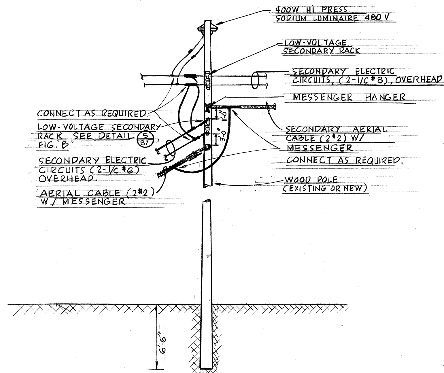
SECONDARY SERVICE - POLE DETAIL (2/87) NTS.
