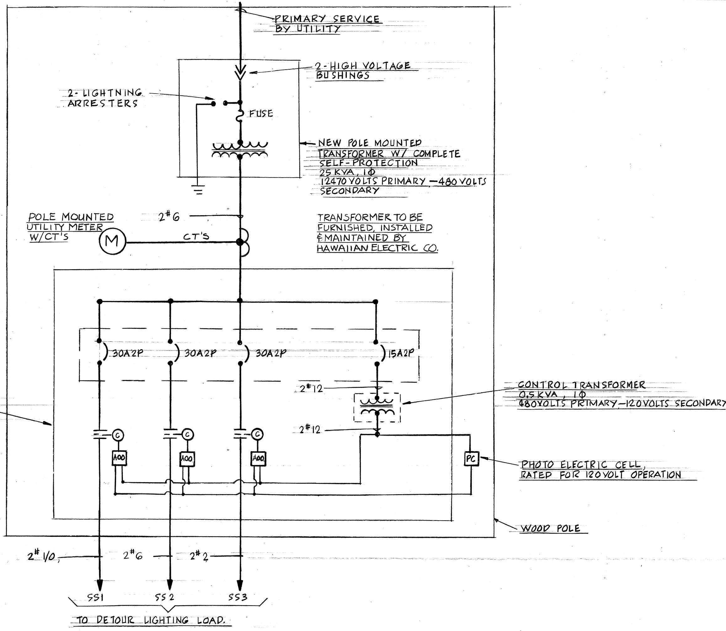
ELECTRICAL-ONE LINE DIAGRAM
