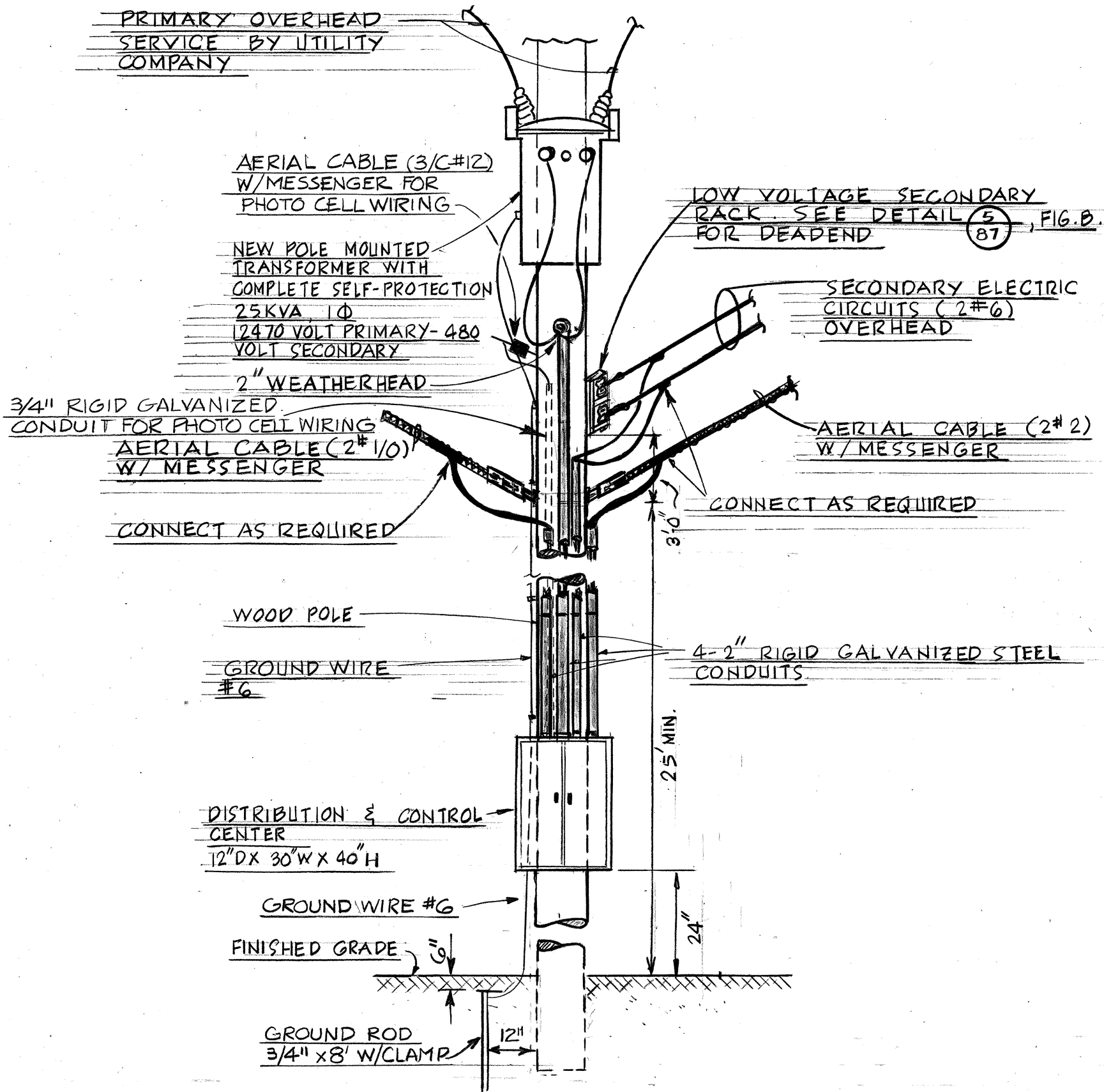
SUB-STATION DETAIL NTS
