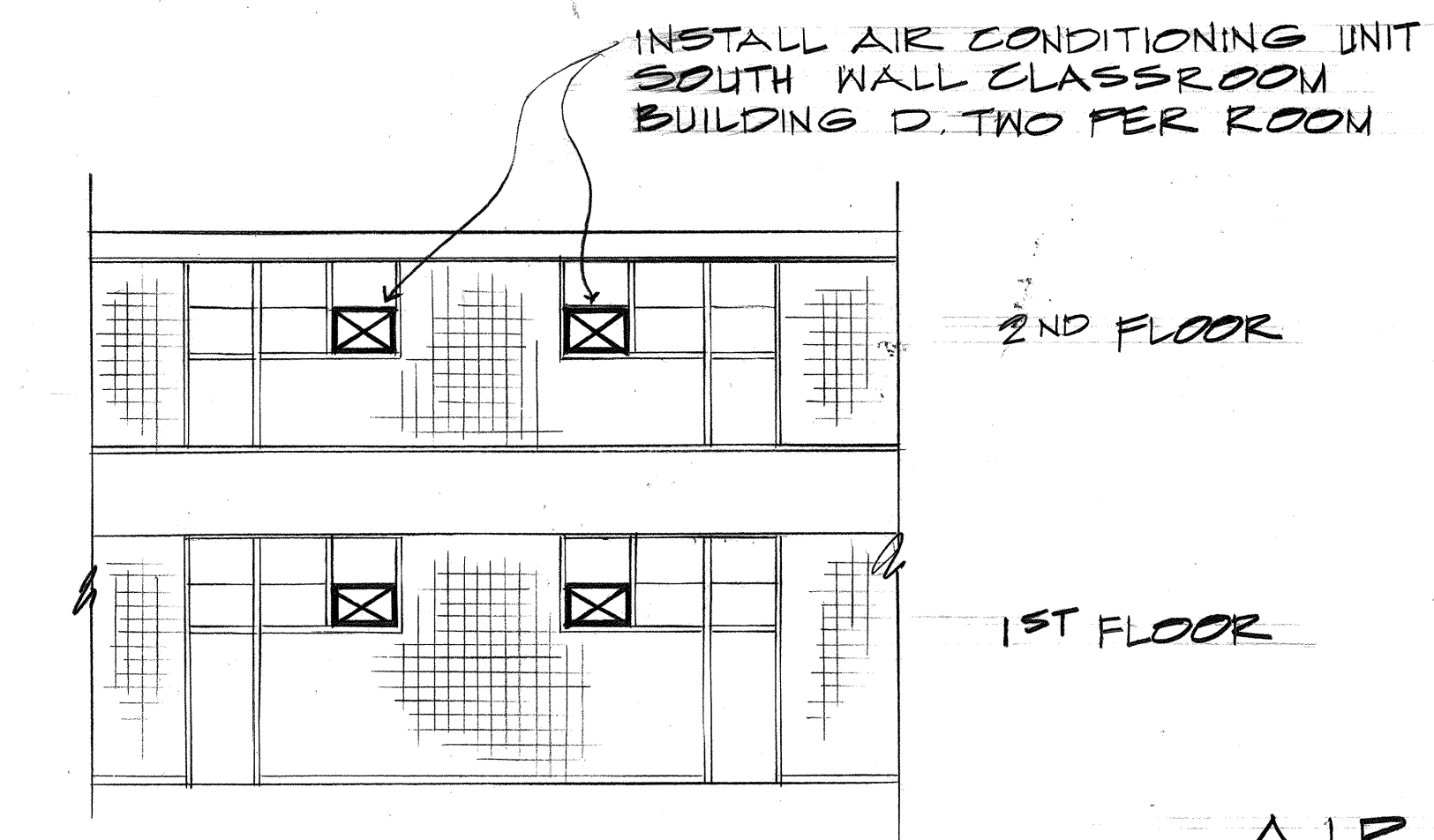
BUILDING D PORTION OF SOUTH ELEVATION SCALE: 1/8"=1'-0"
