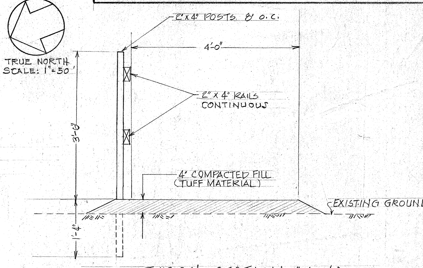
TYPICAL SECTION "A-A" TEMP. PEDESTRIAN WALKWAY SCALE: 3/4" = 1'
