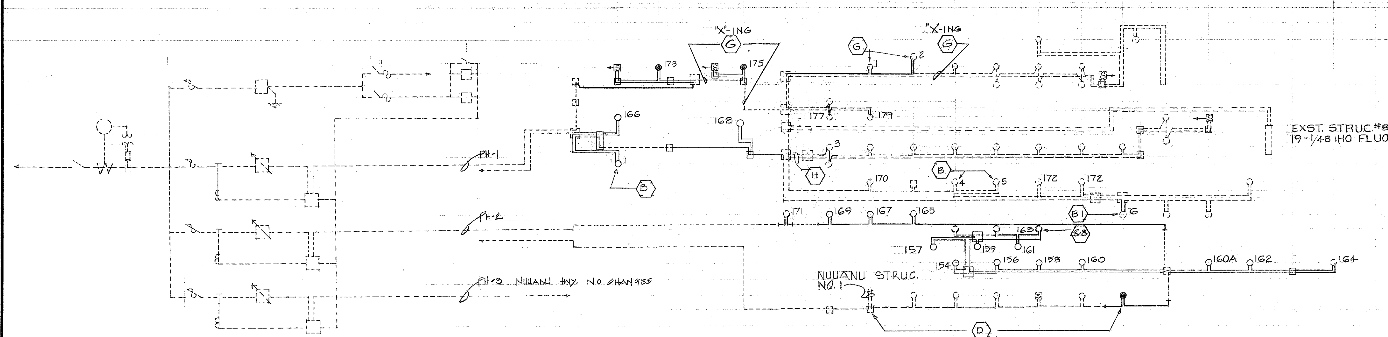
SUBSTATION NO. 2 ONE-LINE DIAGRAM
