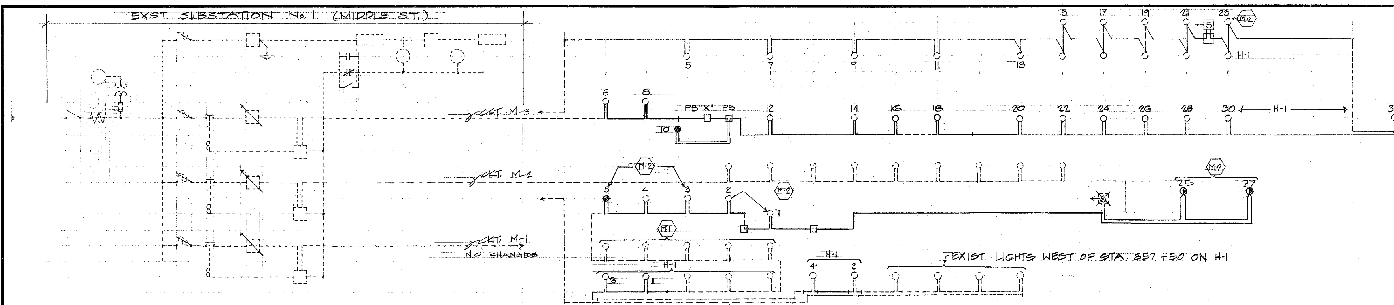
SUBSTATION NO. 1 ONE-LINE DIAGRAM
