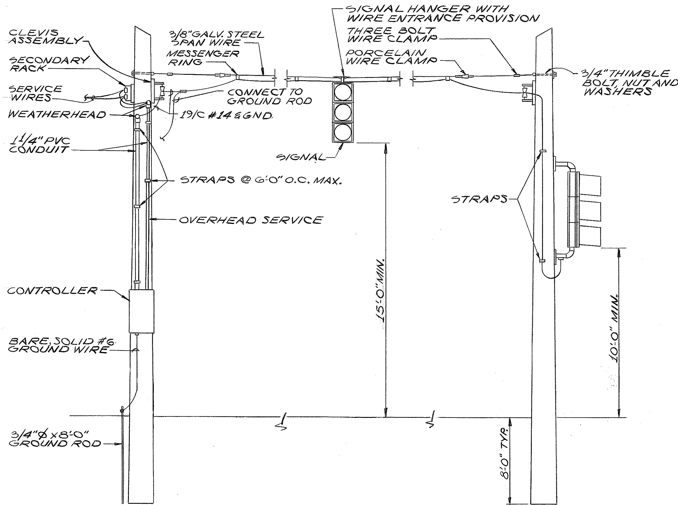
DETAIL 4/5E TRAFFIC SIGNAL FACILITIES N.T.S.
