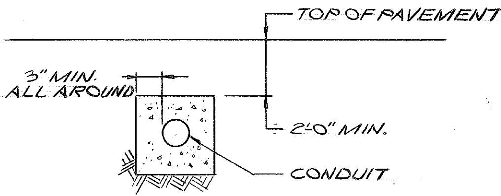
DETAIL 3/5E TRAFFIC SIGNAL SYSTEMS CONDUIT INSTALLATION N.T.S.
