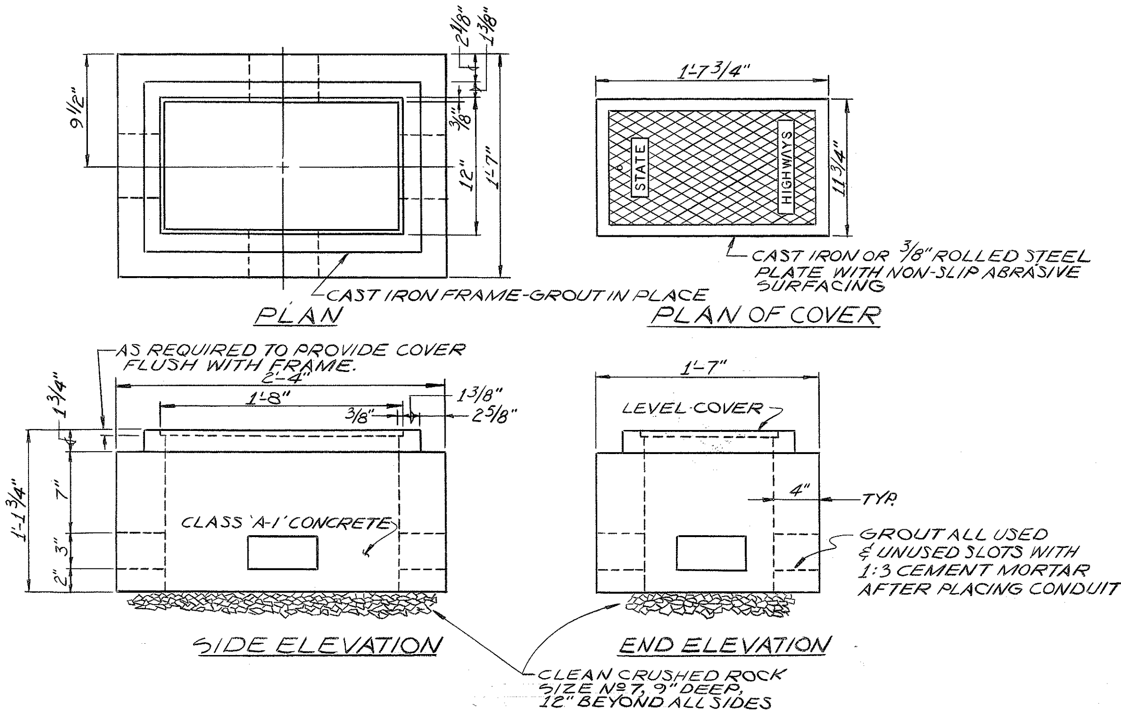
DETAIL 5/5E TYPE 'B' PULL BOX SCALE: 1/4" = 1'-0"
