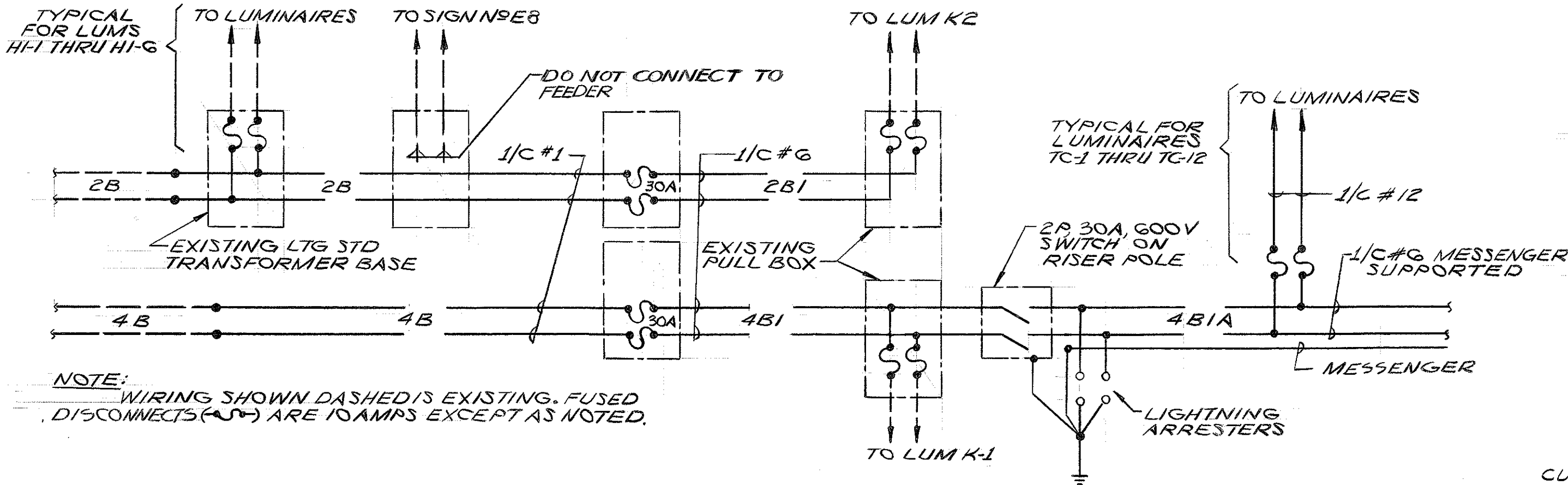
DETAIL 1/5E SCHEMATIC DIAGRAM OF LUMINAIRE CONNECTIONS N.T.S.
