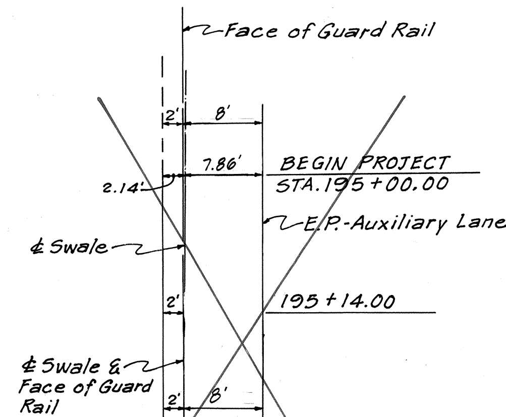
DETAIL A Shoulder, Gutter and Guard Rail Transition To Meet Proposed Construction (By Others) Scale: 1"=10'
