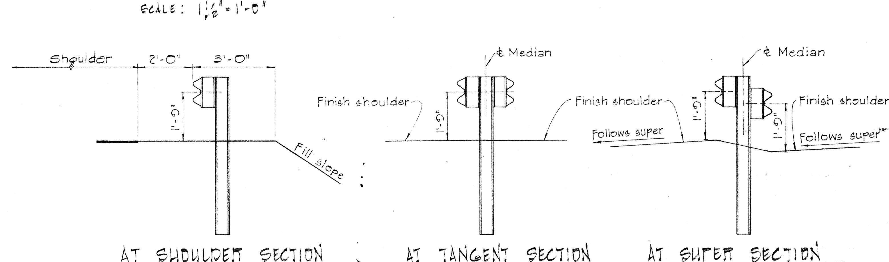
TYPICAL METAL GUARD RAIL DETAIL SCALE: 1/2" = 1'-0"
