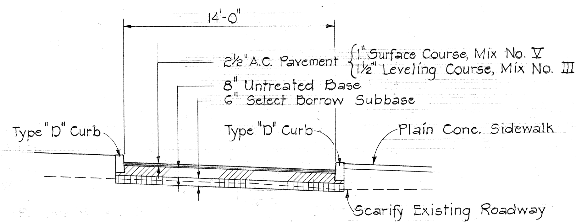
KINAU STREET PAVEMENT SECTION Scale: 1/4" = 1'-0"
