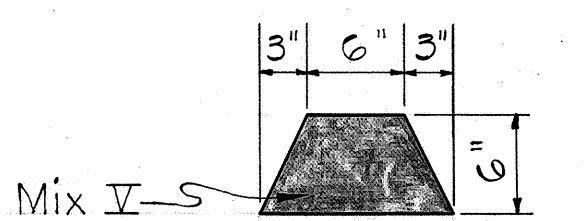
DETAIL OF A.C. CURB Scale: 1"=1'-0"
