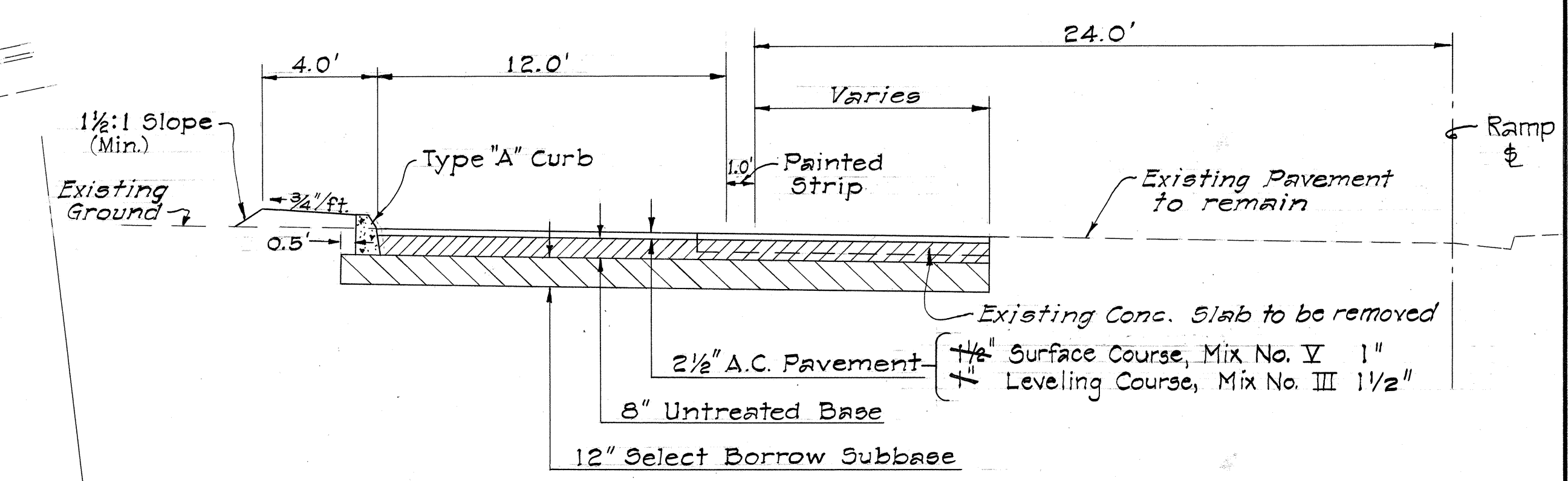
TYPICAL SECTION - RAMP "B" Scale: 1/4" = 1'-0"
