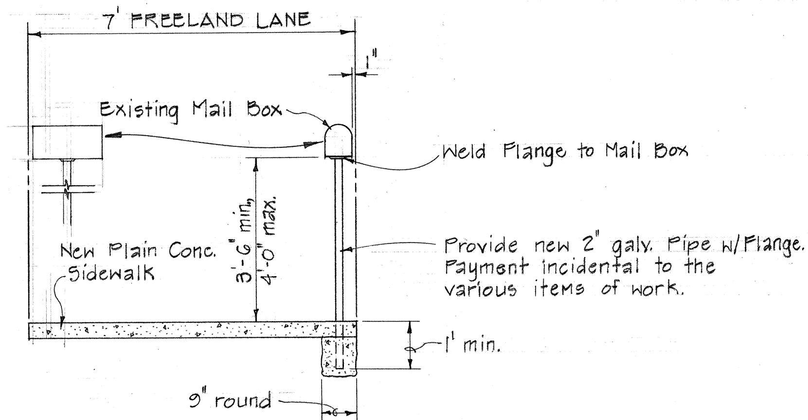
TYPICAL DETAIL FOR MAIL BOX RELOCATION Scale: 1/2" = 1'-0"
