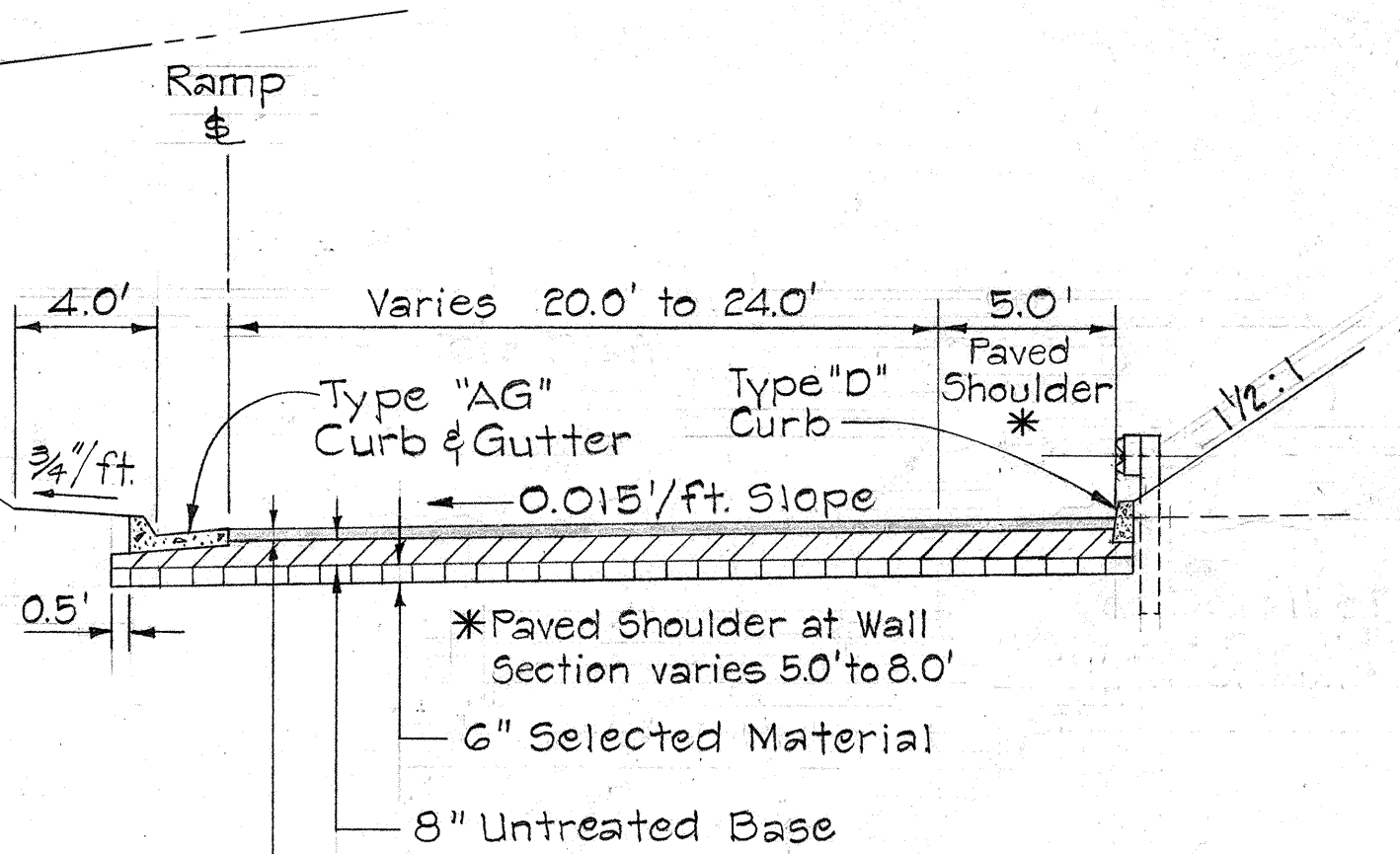
TYPICAL SECTION - RAMP B-1 Scale: 3/16" = 1'-0"
