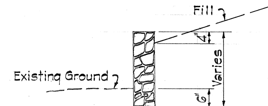
TYPICAL SECTION CRM WALL
