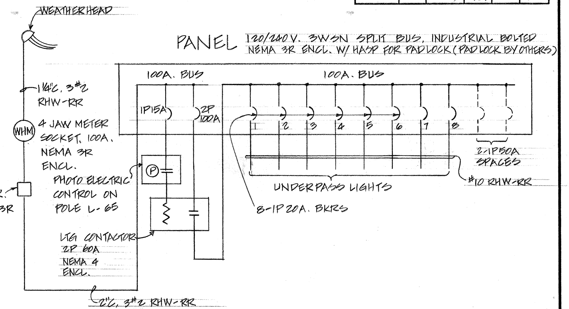
SINGLE LINE DIAGRAM
