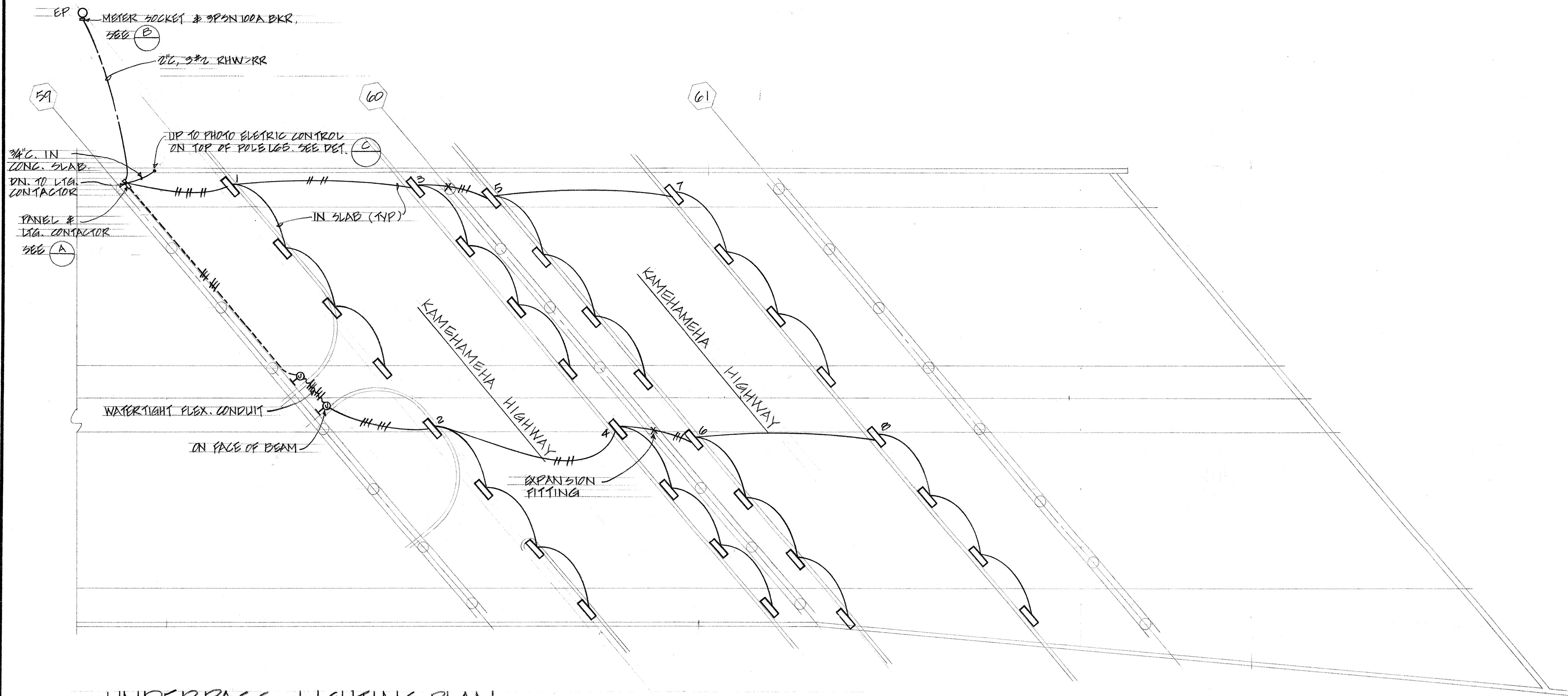
UNDERPASS LIGHTING PLAN SCALE: 1" = 20'-0"
