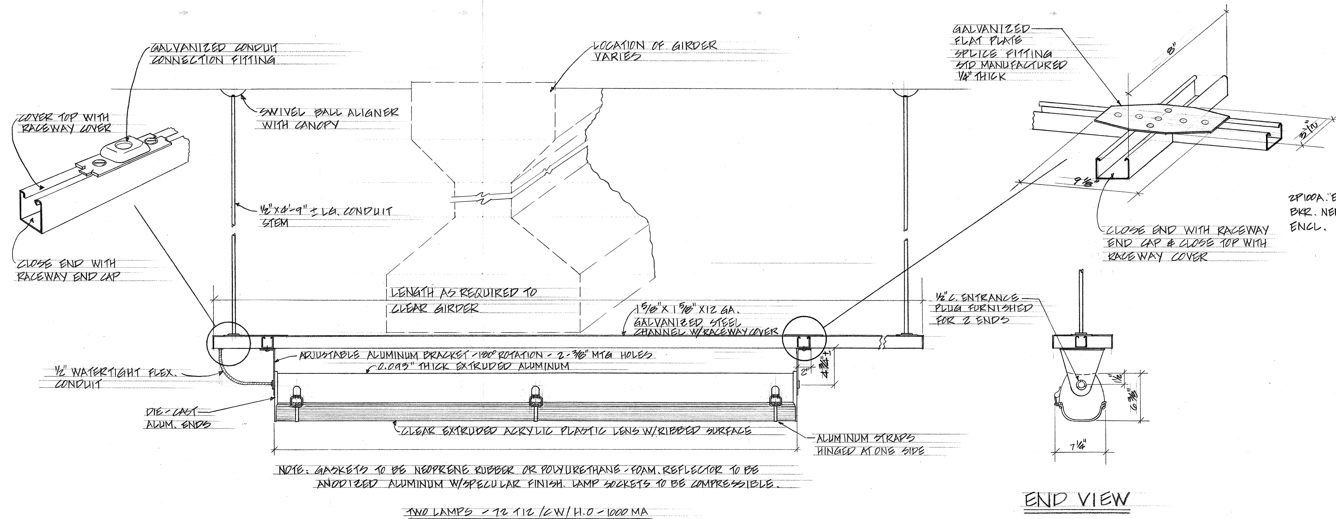
FIXTURE DETAIL-KAMEHAMEHA HWY UNDERPASS
