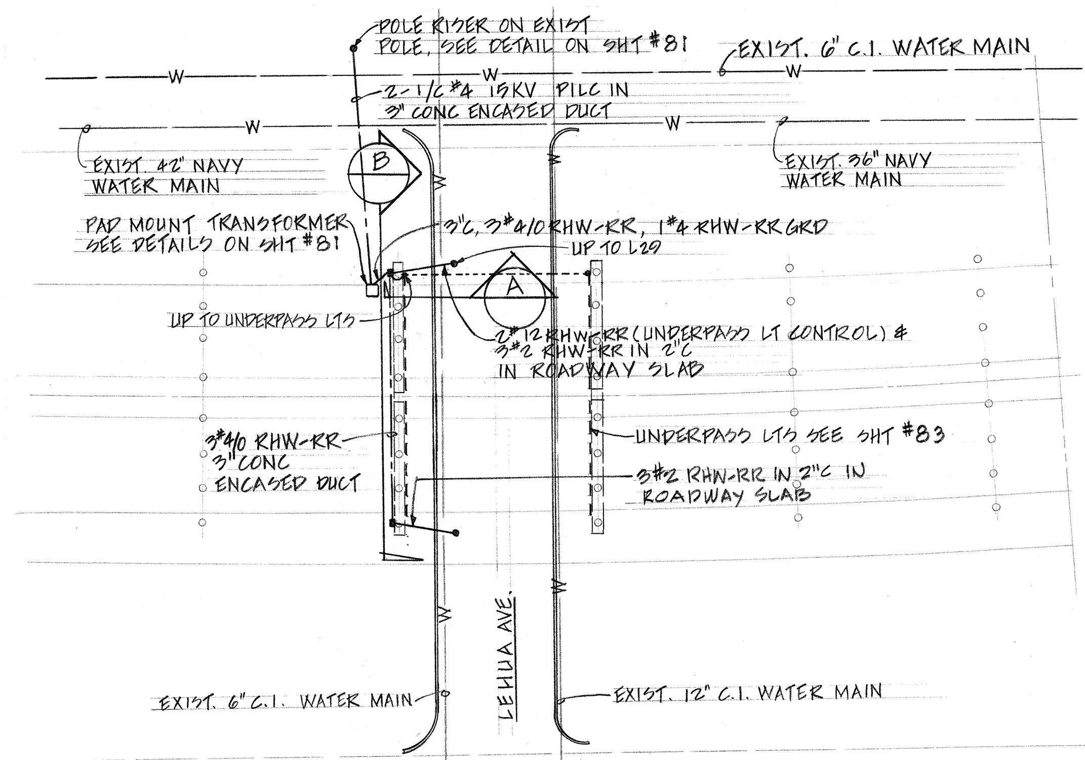
PARTIAL PLAN BELOW VIADUCT SCALE: 1" = 50'
