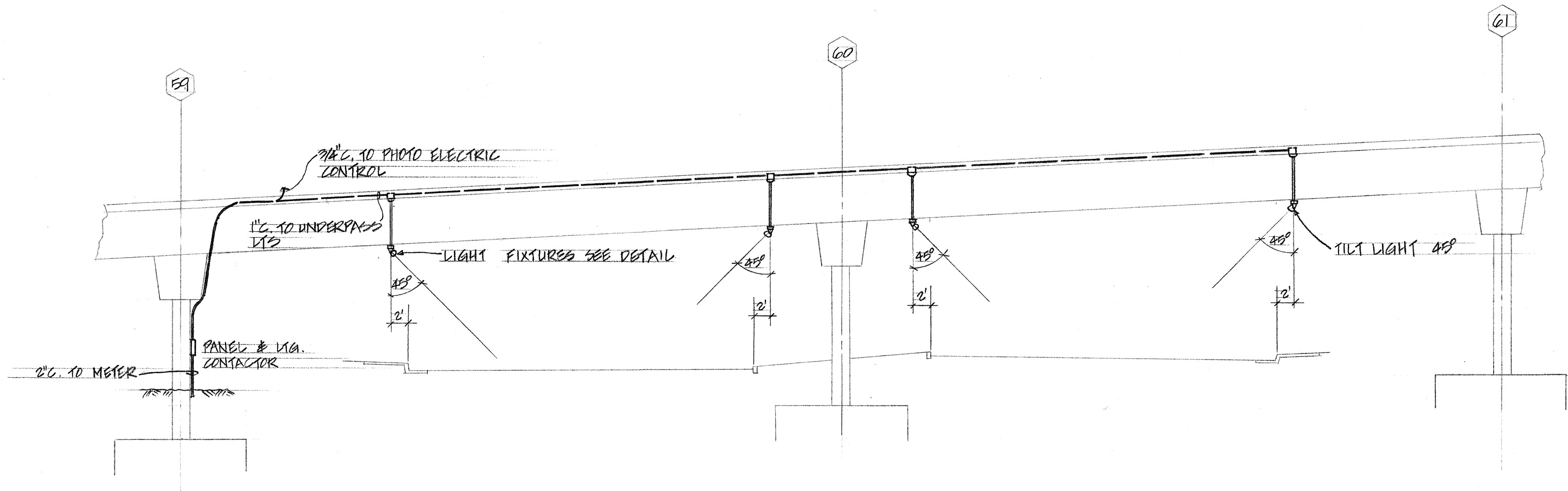
SECTION THRU KAMEHAMEHA HWY SCALE: 1" = 10'-0"
