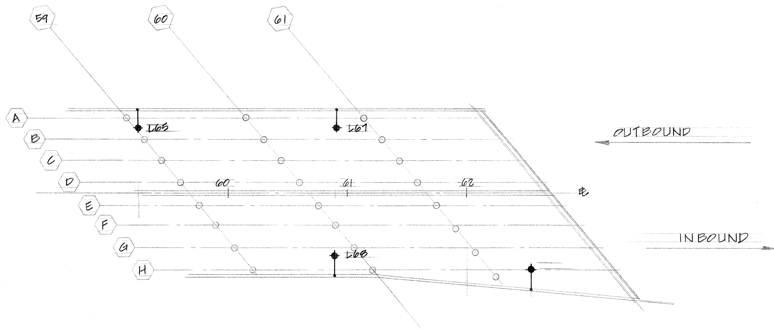
PART. PLAN OF VIADUCT SCALE: 1" = 50'-0"
