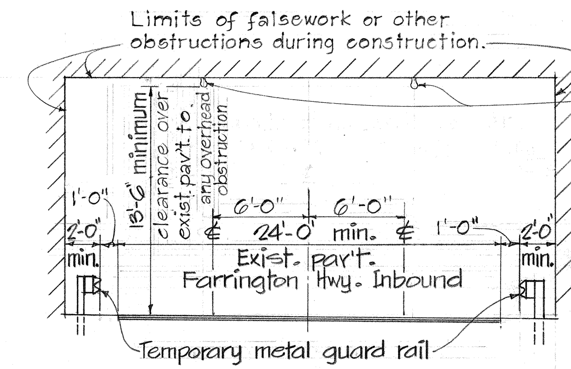
ROADWAY FOR PUBLIC TRAFFIC UNDER STRUCT. #2 DURING CONSTRUCTION, SECT. A Not to Scale
