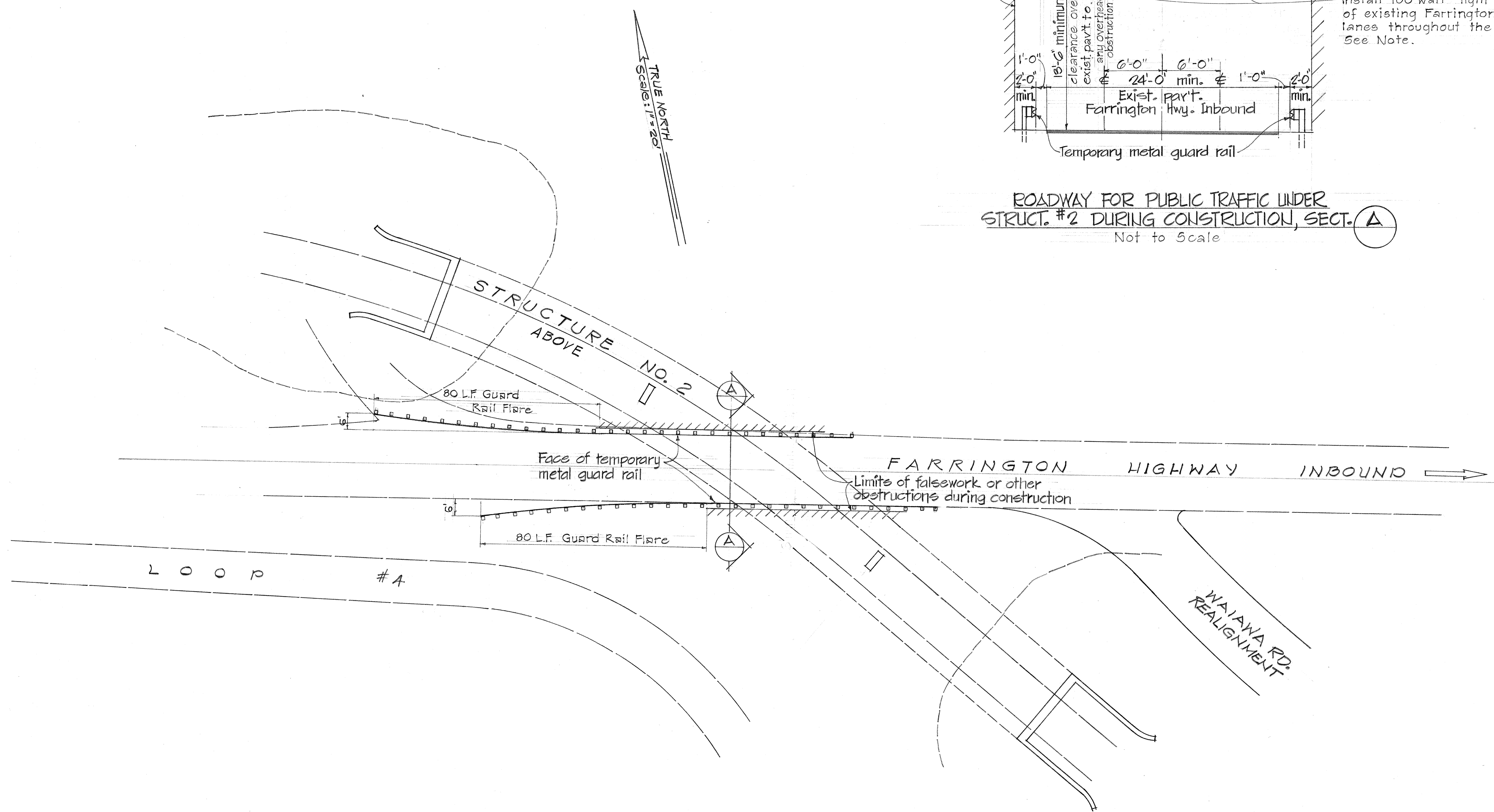
PLAN OF PROVISIONS FOR PUBLIC TRAFFIC AT STRUCTURE NO. 2 DURING CONSTRUCTION
