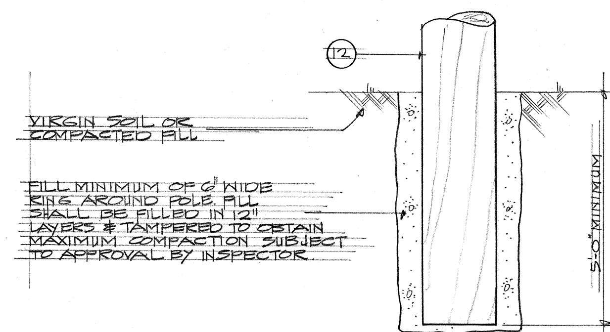
E E-3 POLE SETTING DETAIL NOT TO SCALE
