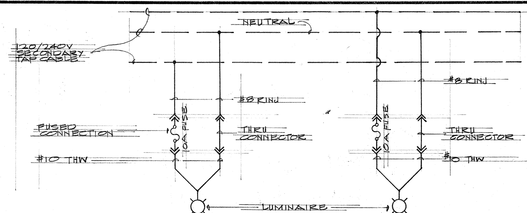
B E-3 TYPICAL STREET LIGHTING CIRCUIT SCHEMATIC DIAGRAM
