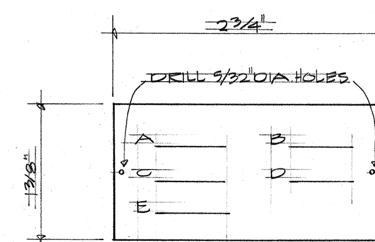
D E-3 IDENTIFICATION TAG DETAIL NOT TO SCALE
