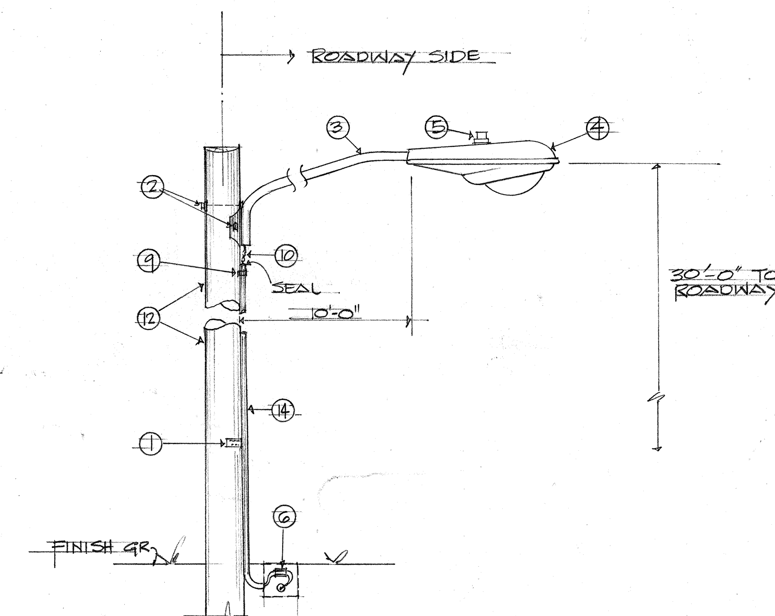
F E-3 DETAIL - STREET LIGHTING WITH UNDERGROUND RISER SERVICE NOT TO SCALE
