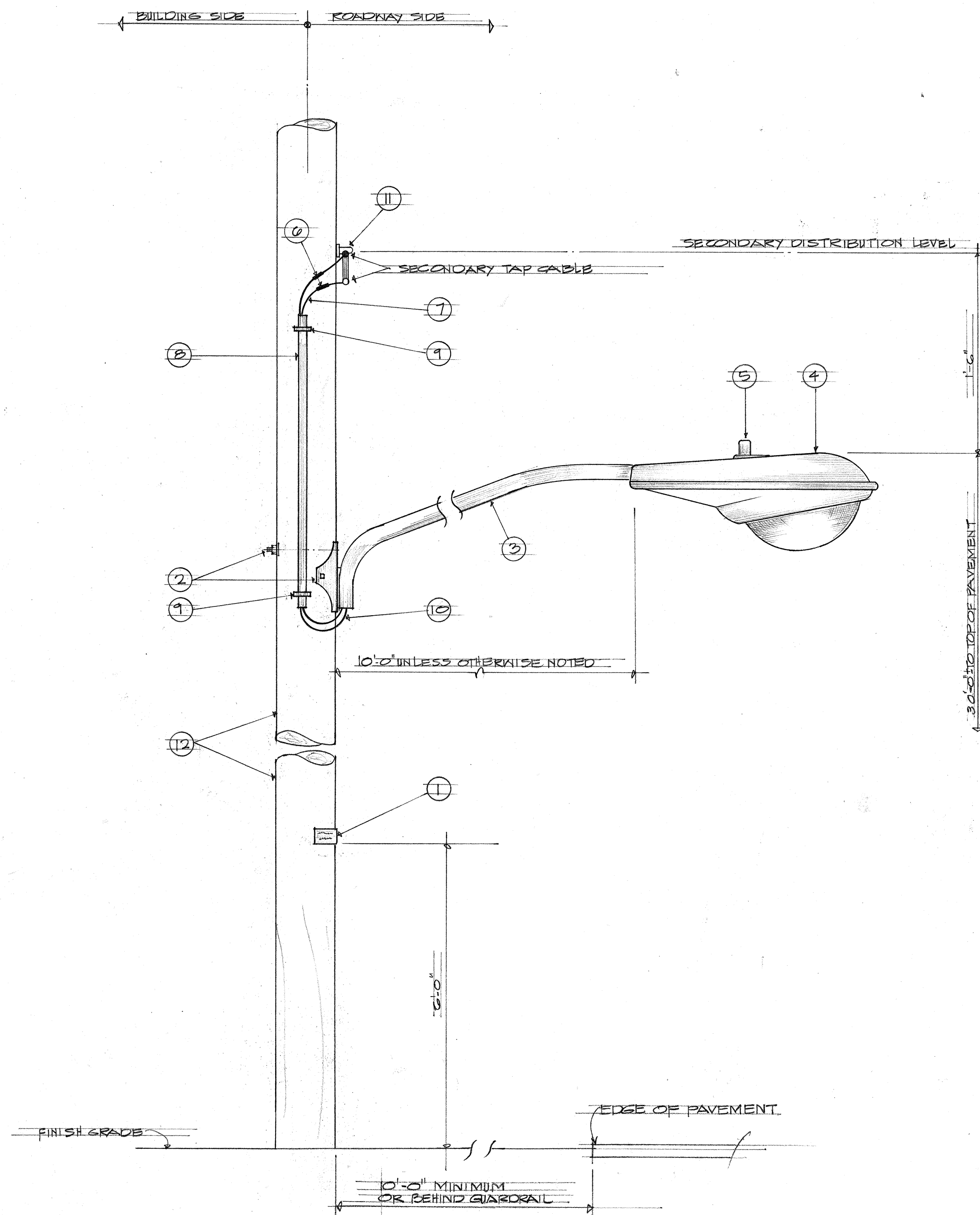
A E-3 STREET LIGHTING CONSTRUCTION DETAIL NOT TO SCALE
