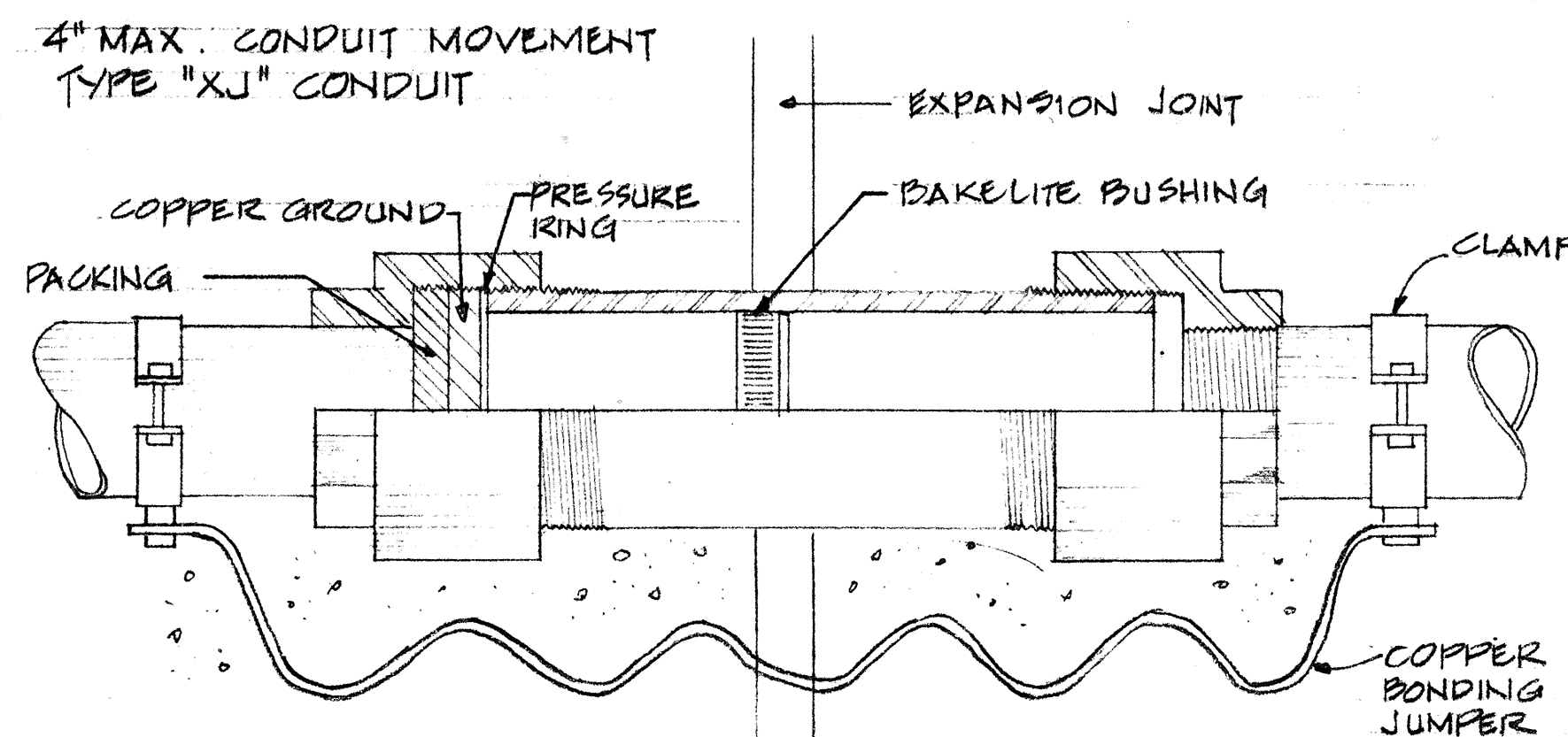
EXPANSION FITTING DETAIL (A) N.T.S.
