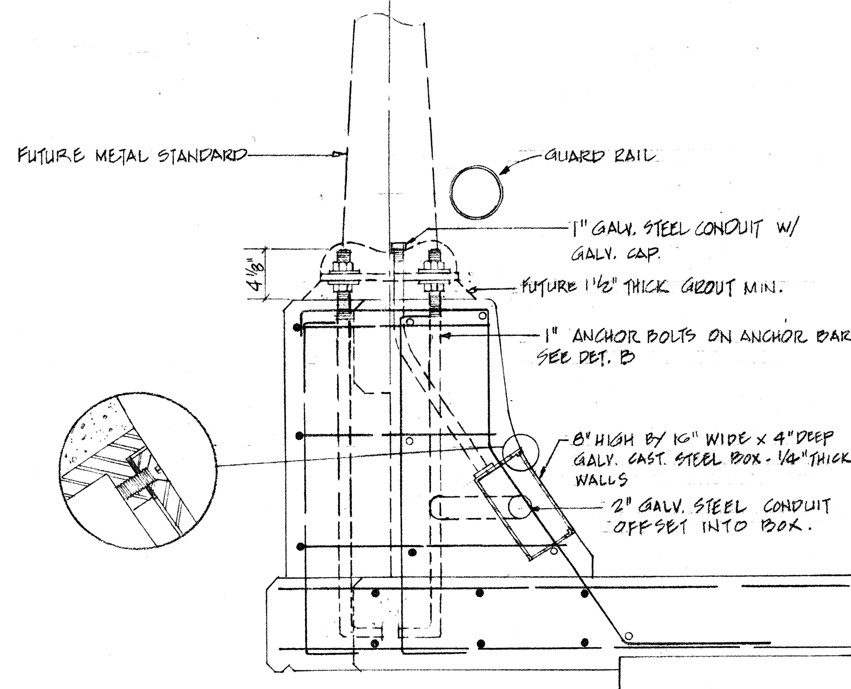
SECTION SCALE: 1 1/2" = 1'-0" TYP. LIGHT BASE DETAILS
