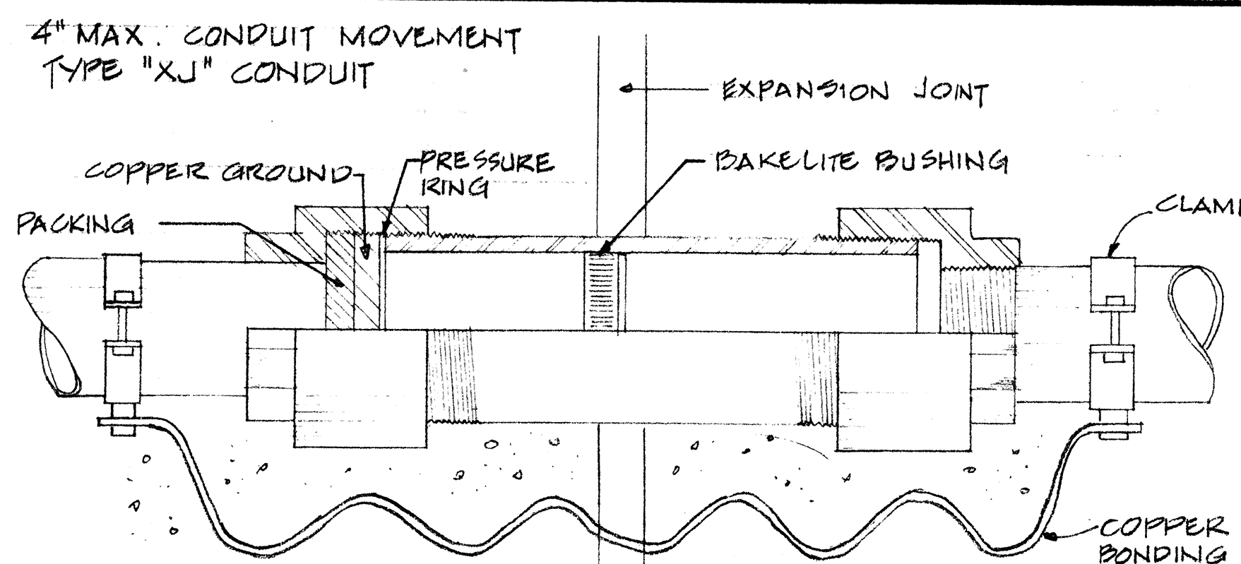
EXPANSION FITTING DETAIL (A) N.T.S.
