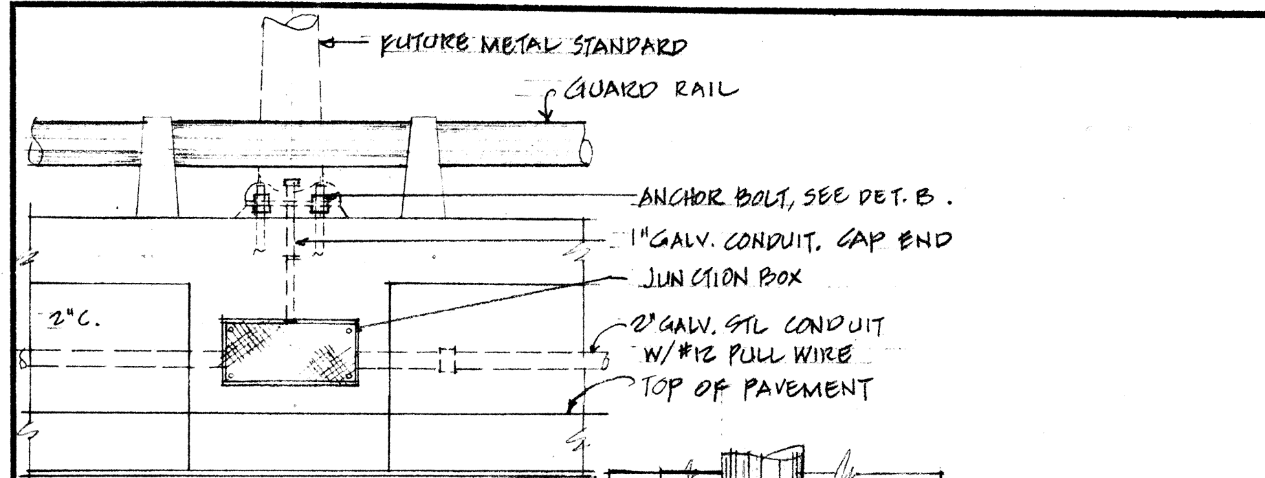
PART ELEVATION SCALE: 3/4" = 1'-0"
