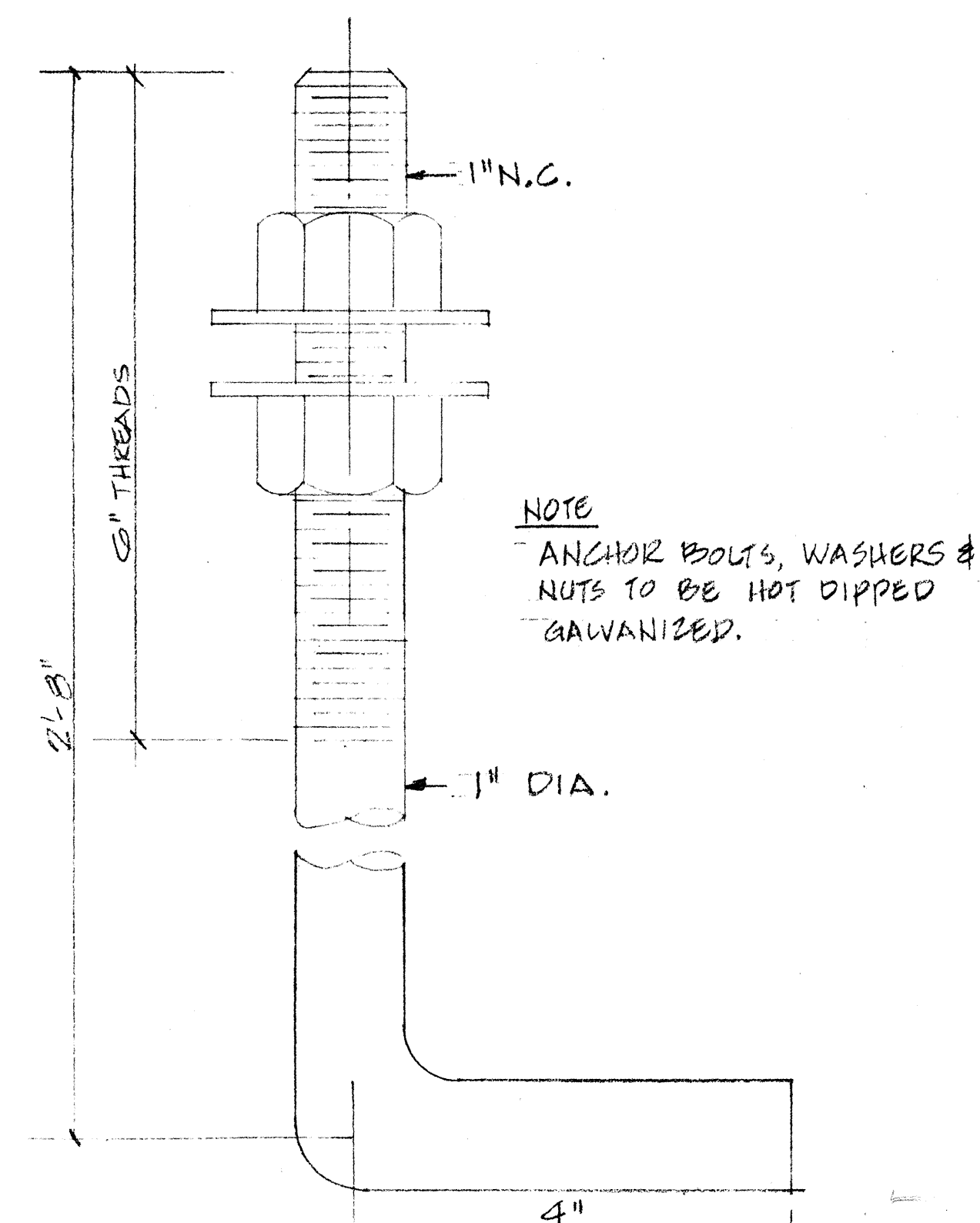
ANCHOR BOLT DETAIL (B) SCALE: 3/4" = 1"
