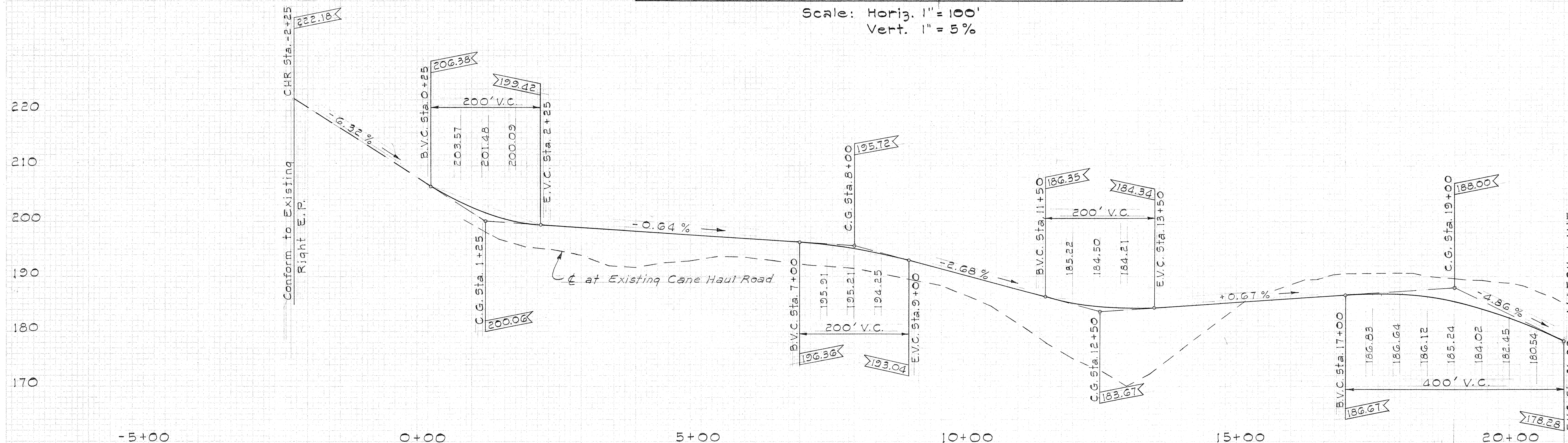
PROFILE CANE HAUL ROAD "A"
