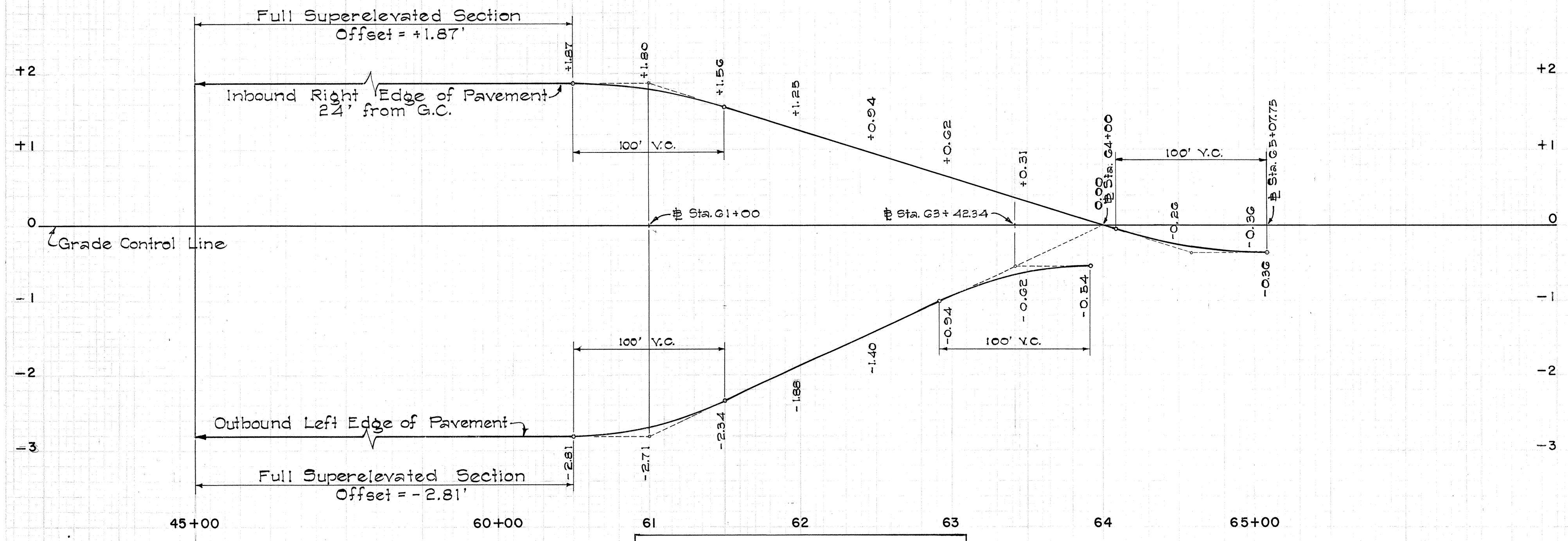
CURVE B1 SE = 0.078 / FT.
