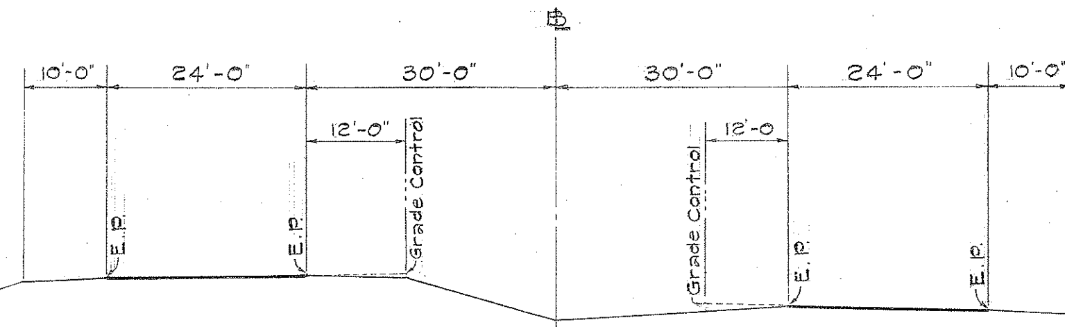
TYPICAL SECTION OF ROADWAY Scale: 1/2" = 1'-0"
