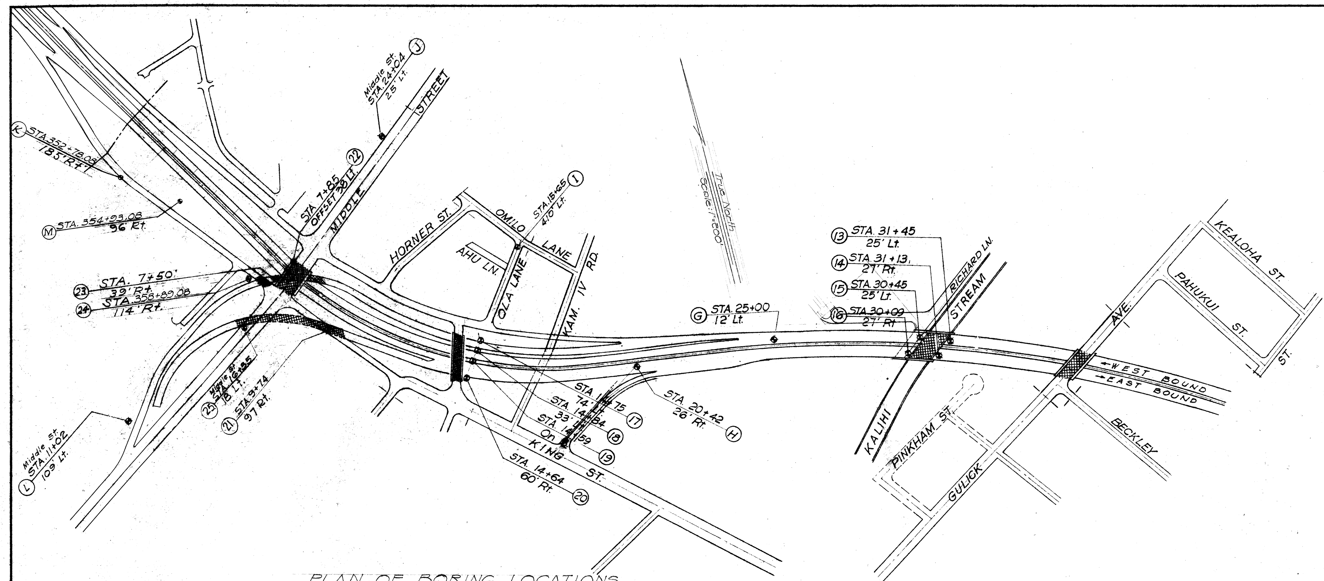
PLAN OF BORING LOCATIONS Scale: 1"=200'
