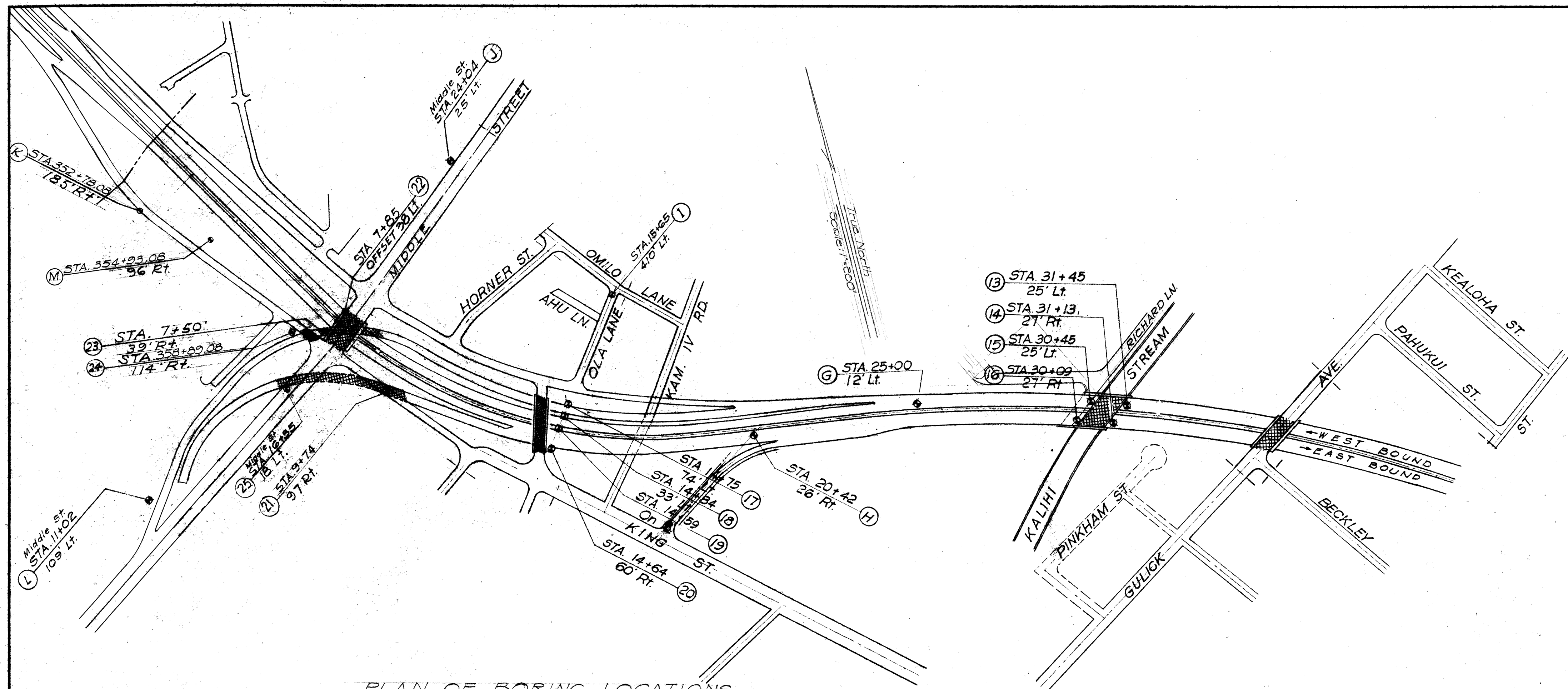
PLAN OF BORING LOCATIONS Scale: 1"=500'
