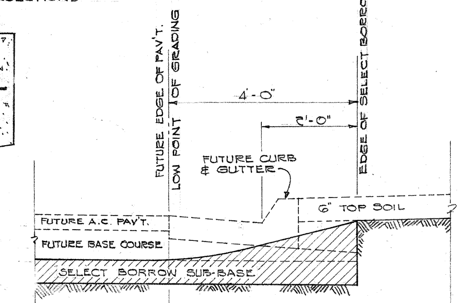
TYPICAL SECTION SHOWING LOW POINT OF GRADING AND BUILT-UP SELECT BORROW SCALE: 1/2" = 1'-0"
