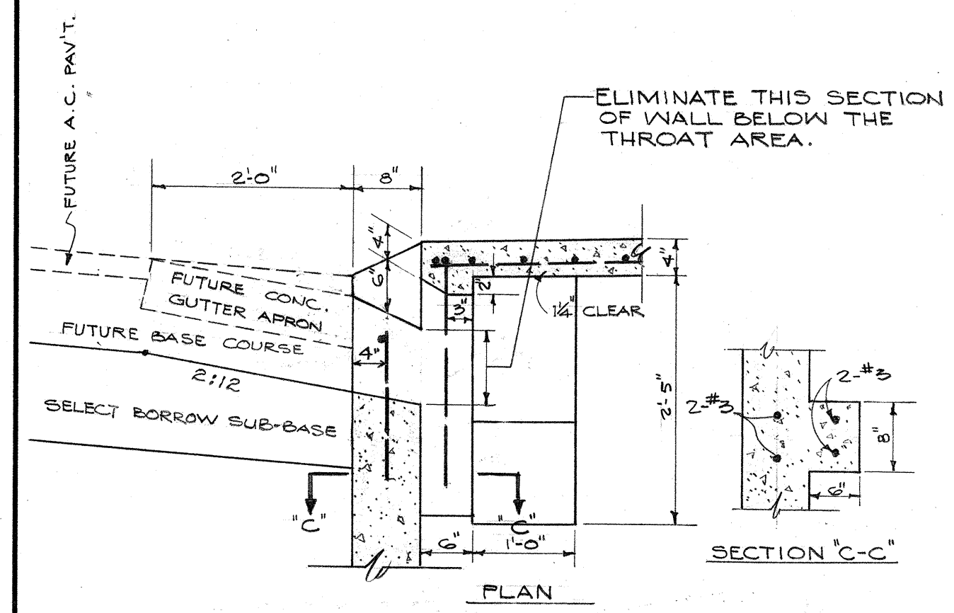
REVISED THROAT DETAIL FOR TYPE "EG" CURB & GUTTER SCALE: 3/4" = 1'-0"
