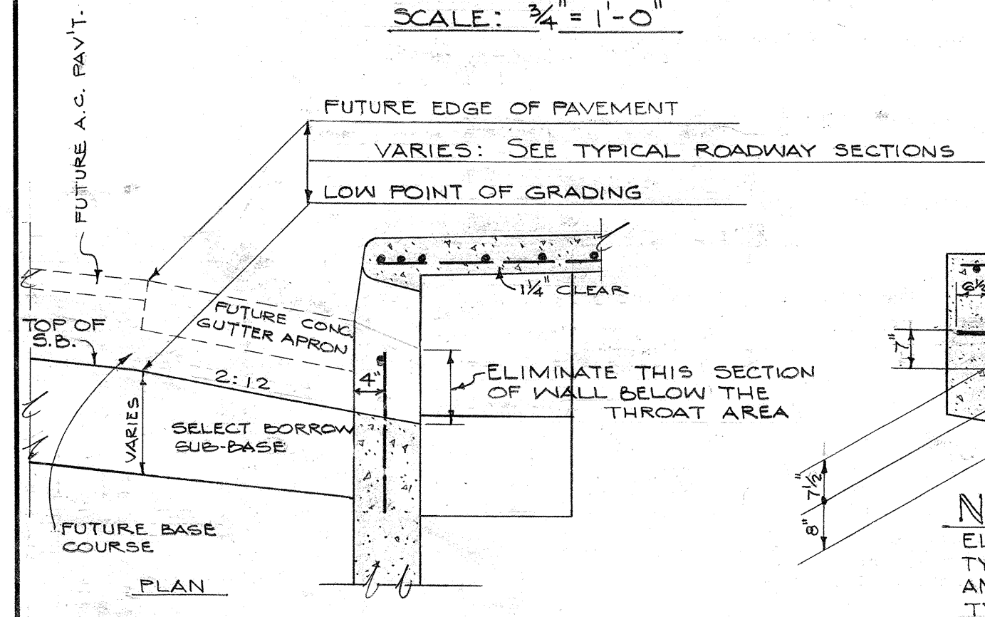
REVISED THROAT DETAIL FOR TYPE "DG" CURB & GUTTER SCALE: 3/4" = 1'-0"
