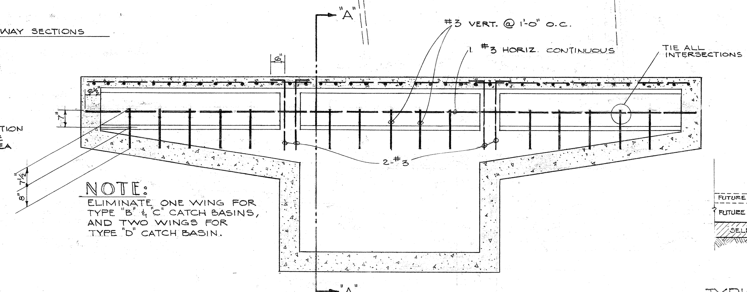
REVISED THROAT DETAILS FOR TYPE "A" CATCH BASINS (TO BE USED WHERE FINISHED GRADE IS AT TOP OF SELECT BORROW SUB-BASE) SCALE: 1/2" = 1'-0"
