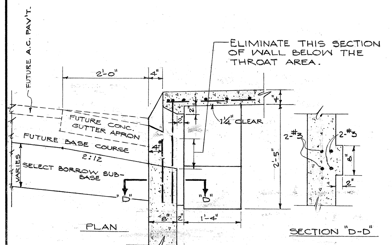
REVISED THROAT DETAIL FOR TYPE "AG" CURB & GUTTER SCALE: 3/4" = 1'-0"
