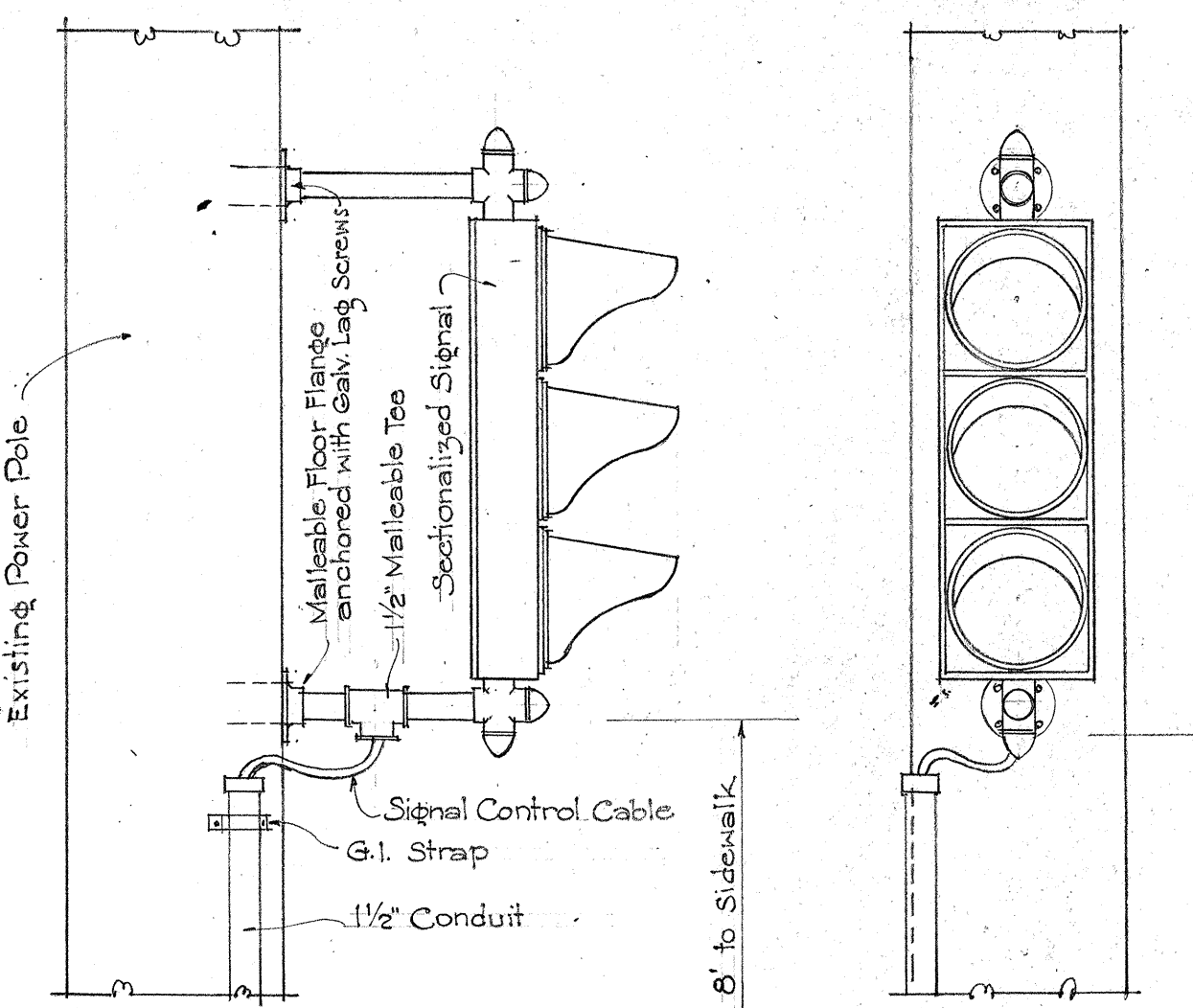
FRONT VIEW
