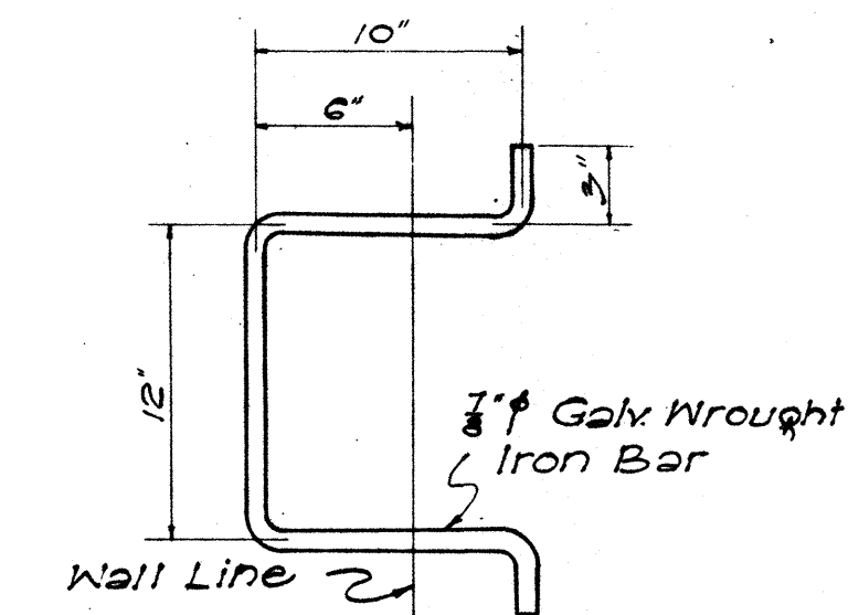
MANHOLE RUNG
