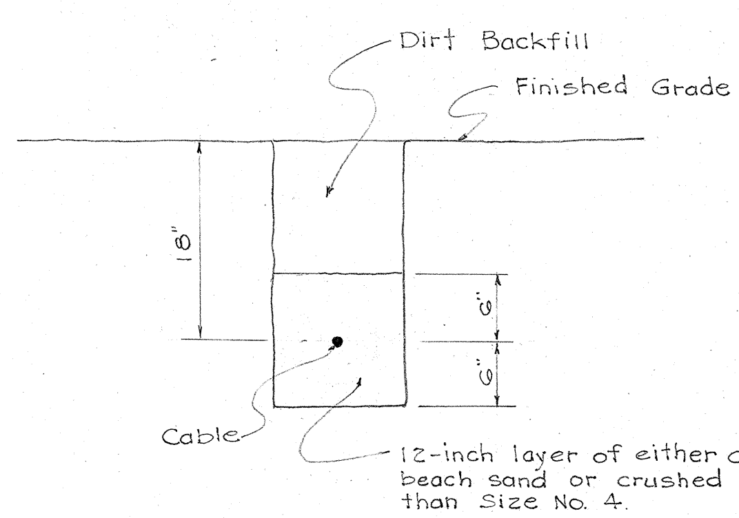
TRENCH AND BACKFILL FOR DIRECT BURIAL CABLE Scale: 1/2" = 1'-0"
