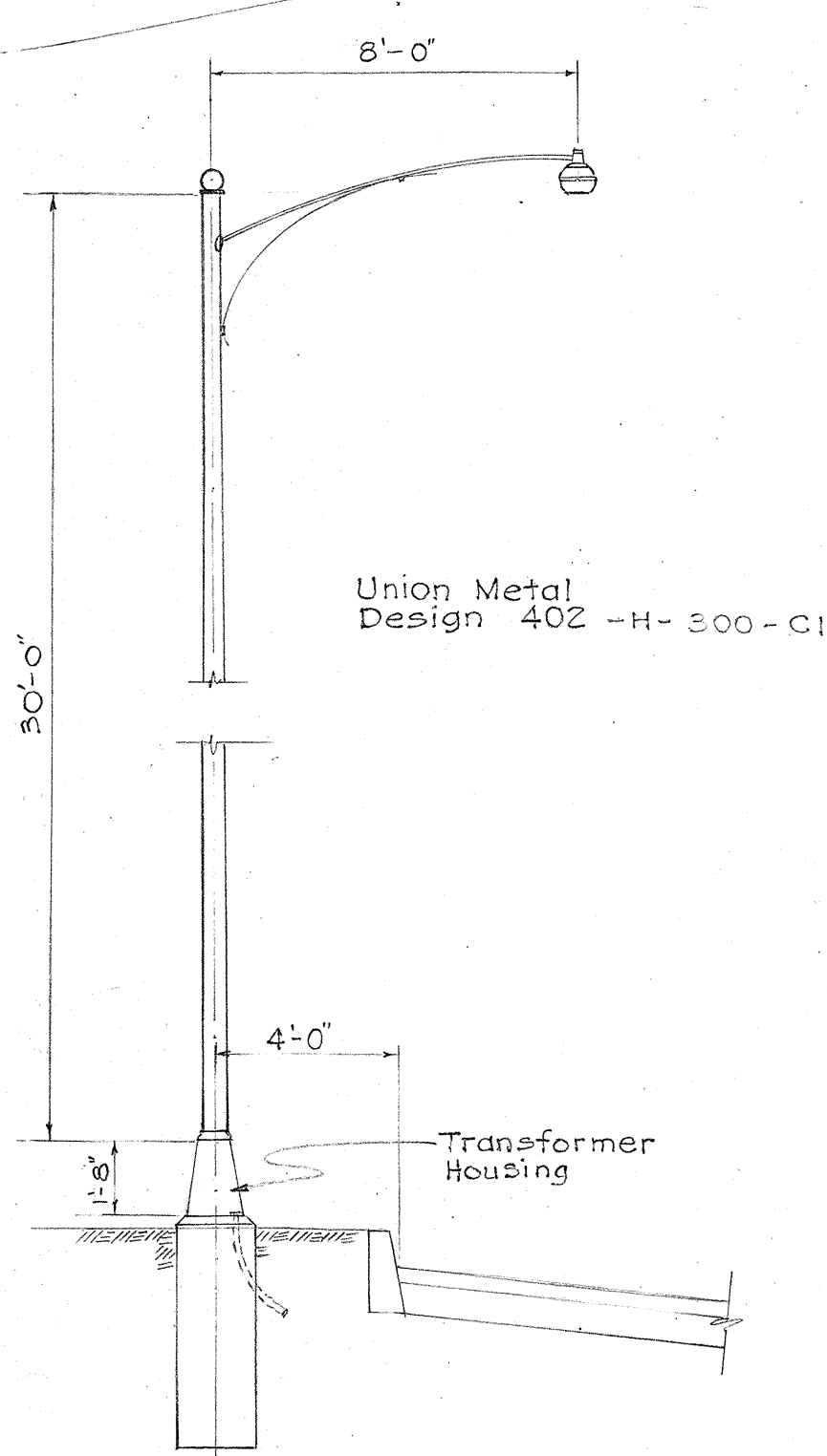
LIGHTING STANDARD Scale: 1/4" = 1'-0"
