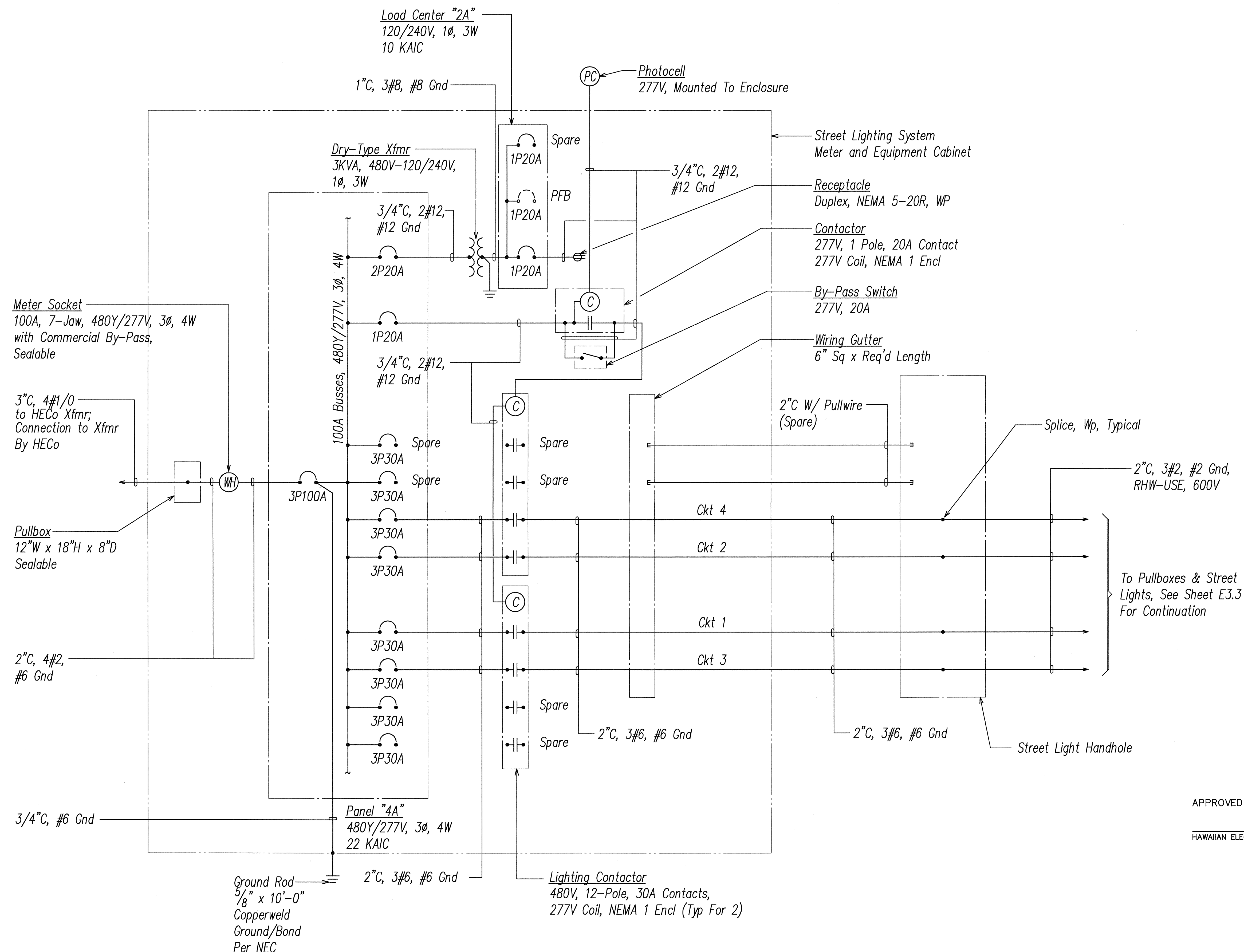
STREET LIGHTING SYSTEM "A" ONE-LINE DIAGRAM
