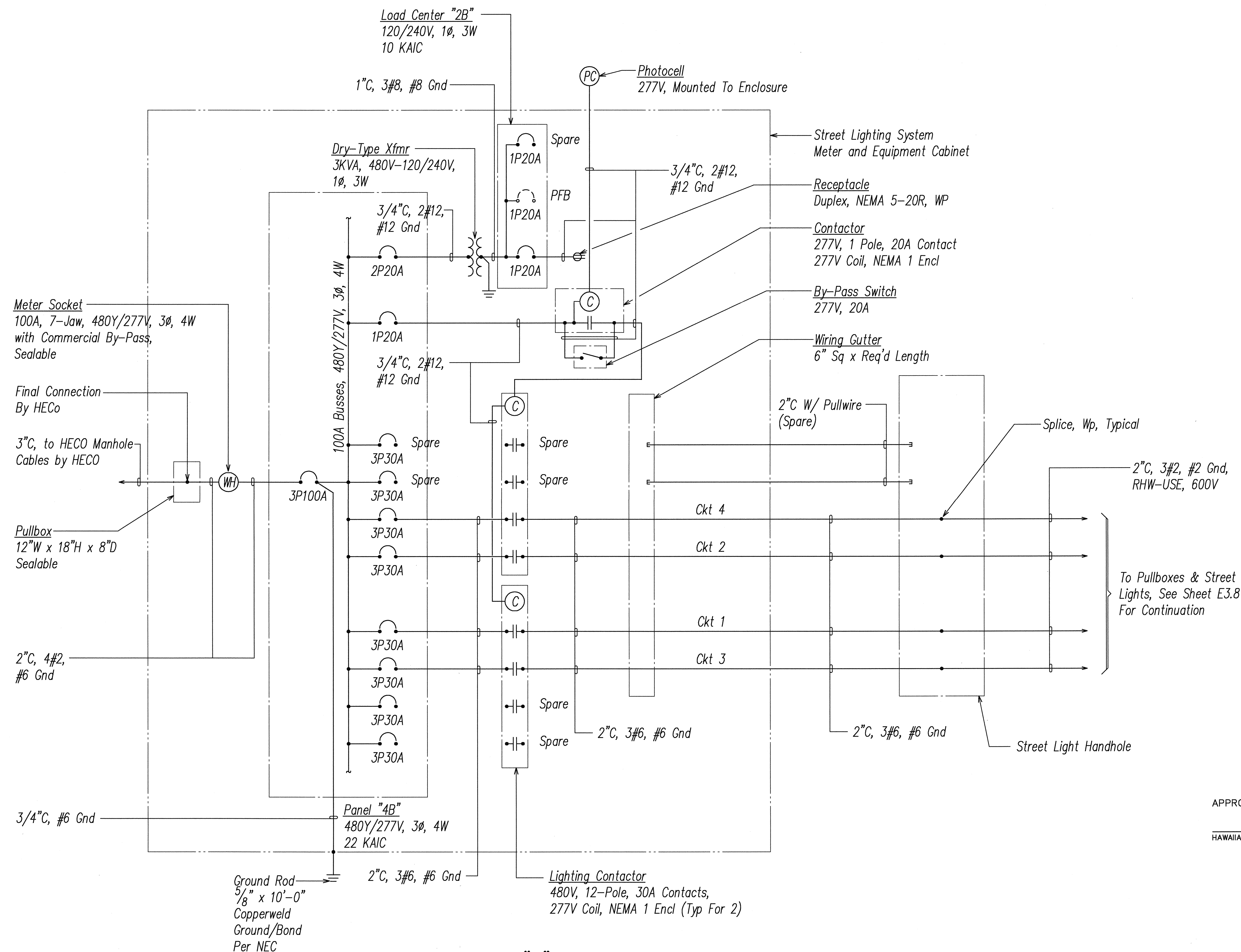
STREET LIGHTING SYSTEM "B" ONE-LINE DIAGRAM
