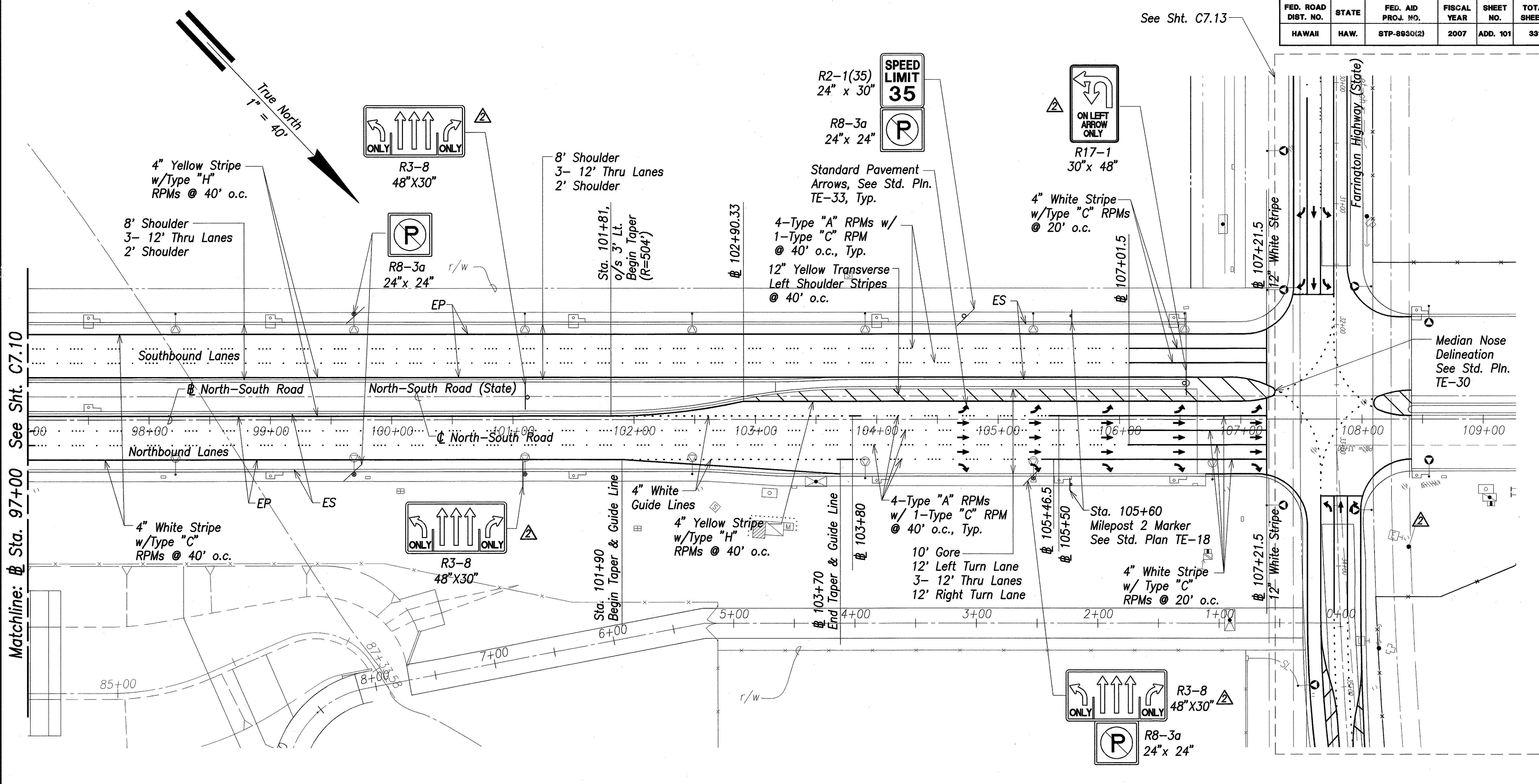
Striping Plan - @ Sta. 97+00 to Farrington Highway Scale: 1" = 40'
