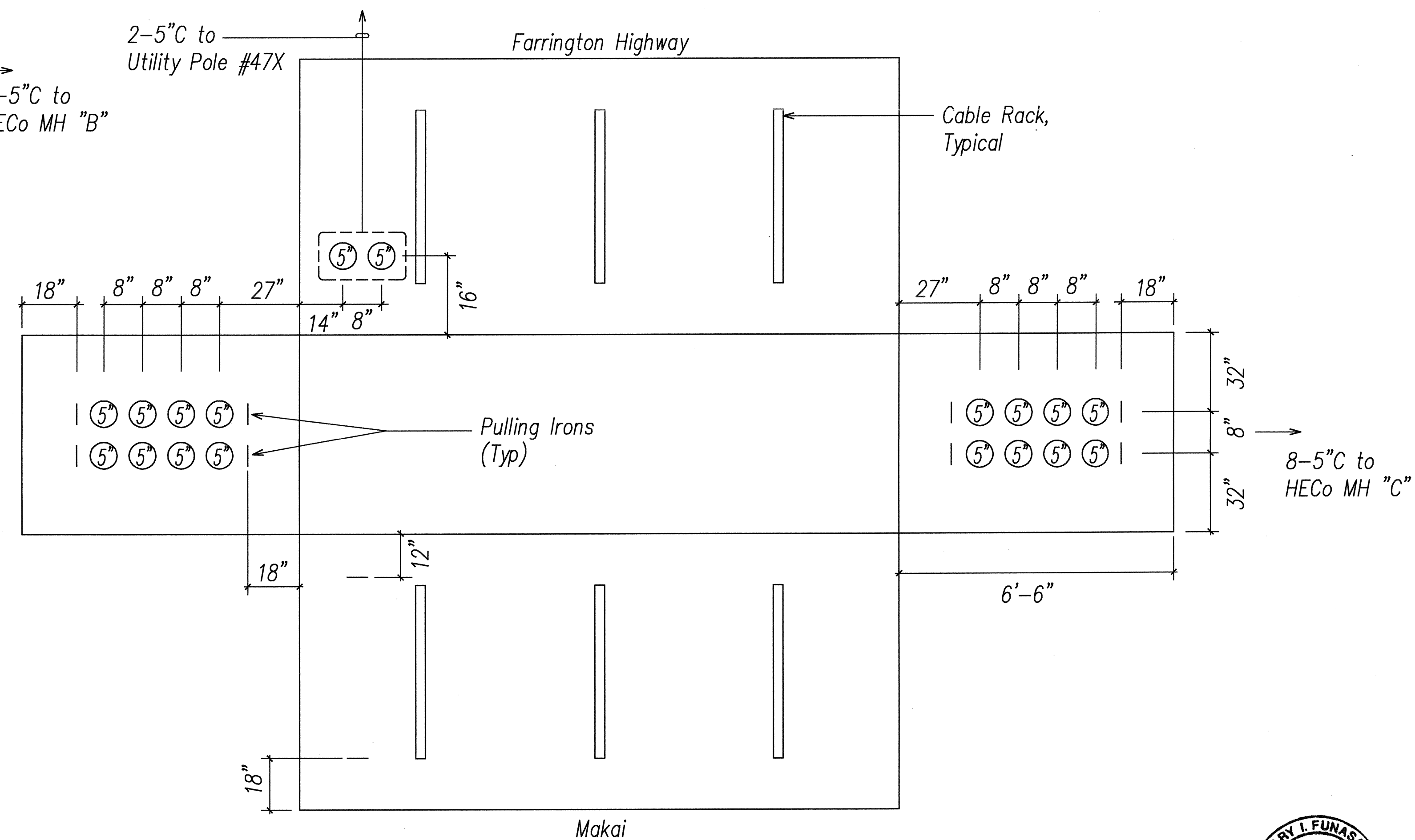
HECO 6' X 14' MANHOLE "B"
