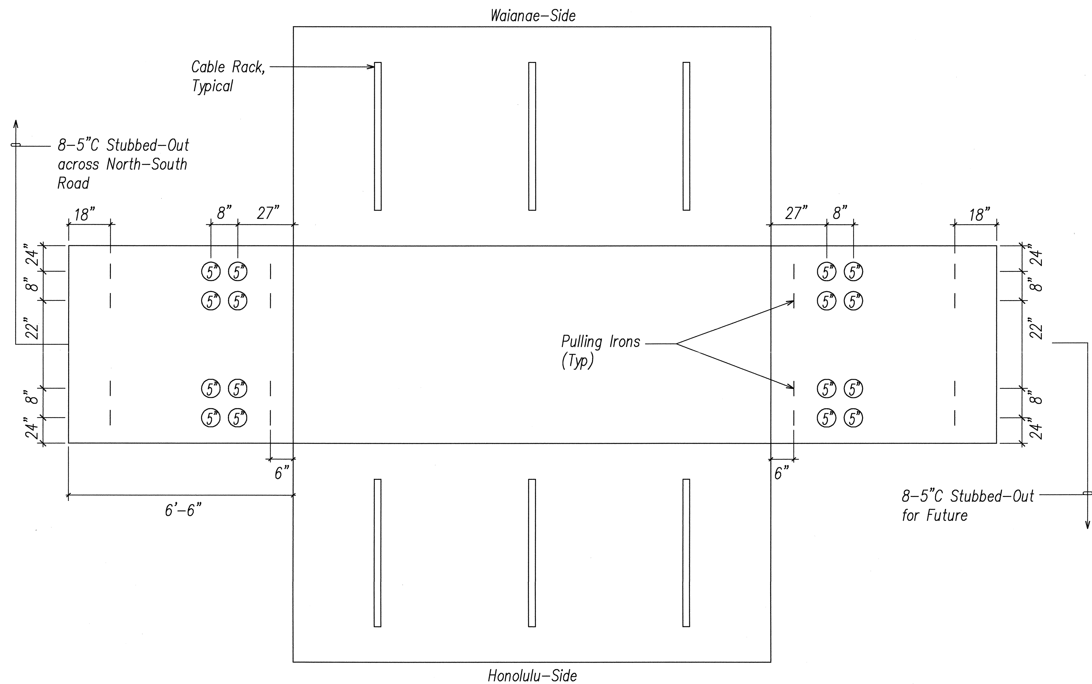
HECO 7' X 16' MANHOLE "2"
