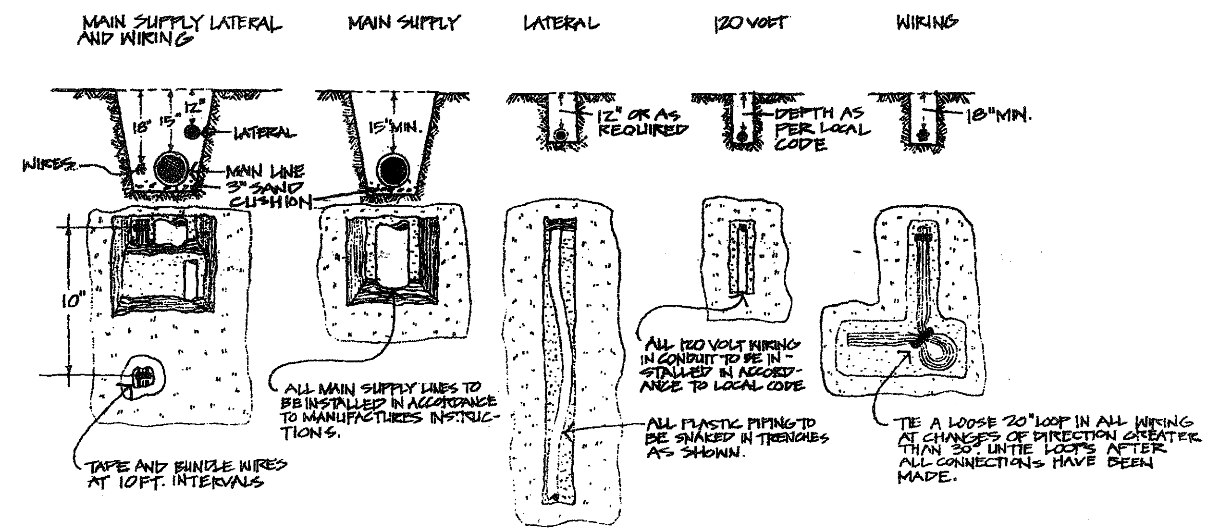
TYPICAL TRENCHING DETAILS NO SCALE
