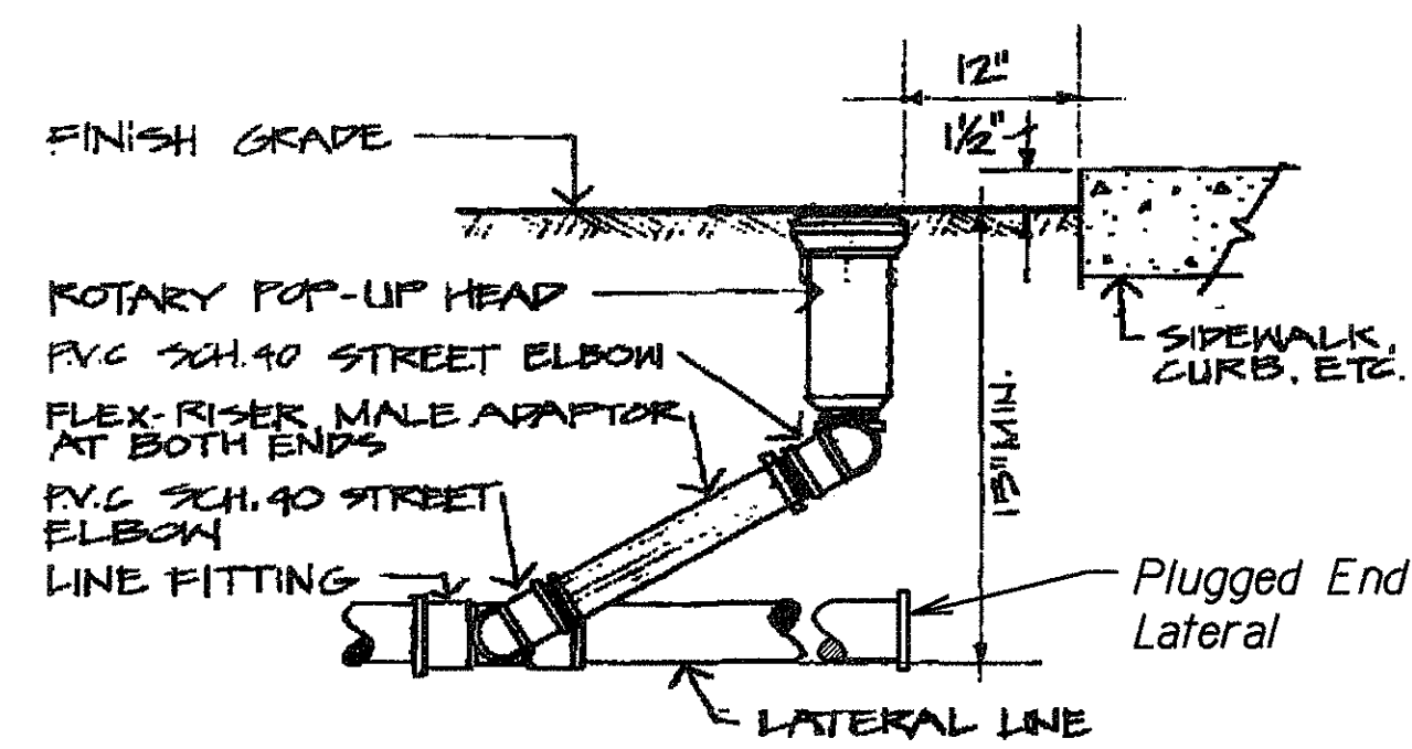
ROTARY POP-UP HEAD DETAIL NO SCALE
