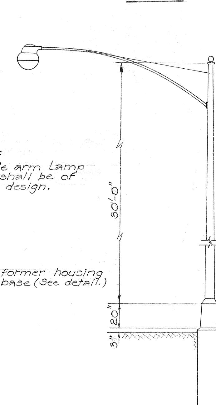
TYPICAL SINGLE ARM METAL LAMP POST Scale: 1/4"=1'-0"
