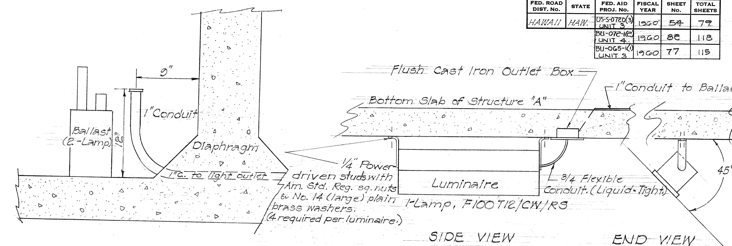
DETAIL OF BALLAST IN STRUCTURE CELL
