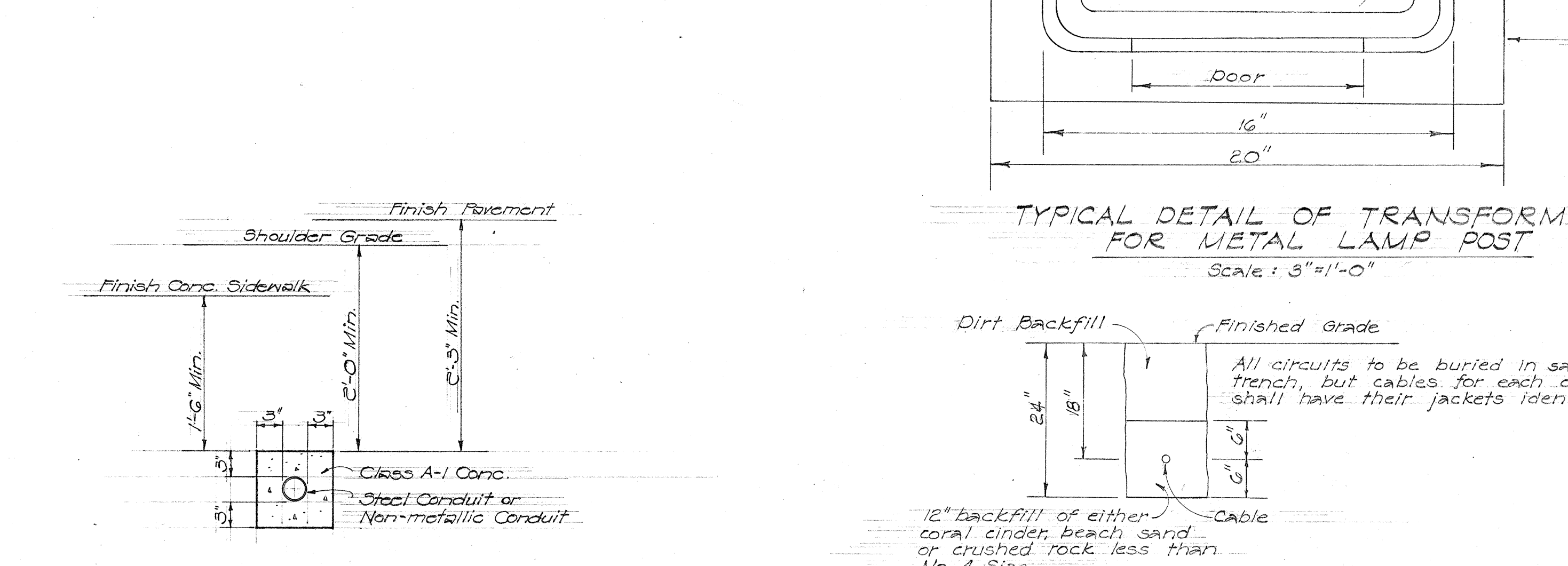
TYPICAL DETAIL OF CONDUITS ENCASED IN CONCRETE JACKET Scale: 1"=1'-0"
