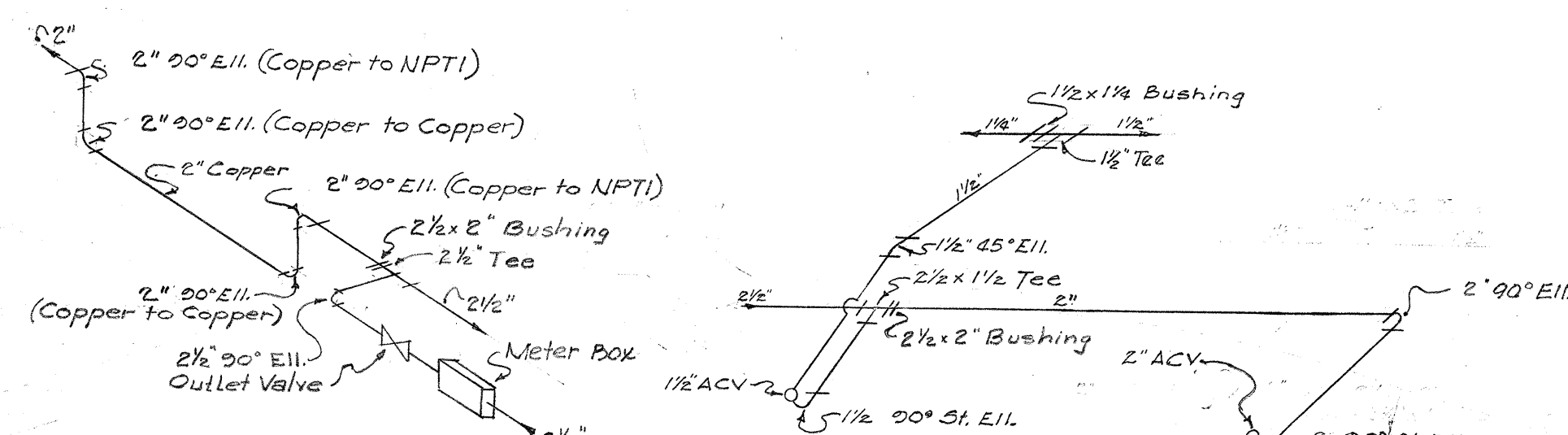
DETAIL 3-J
