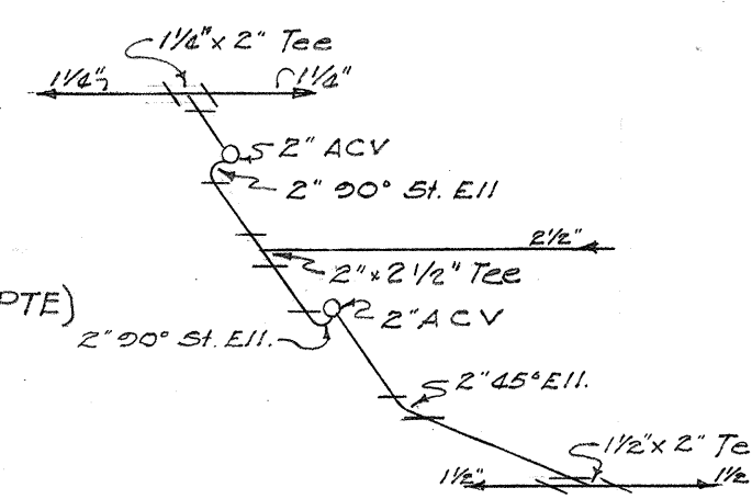
DETAIL 3-C
