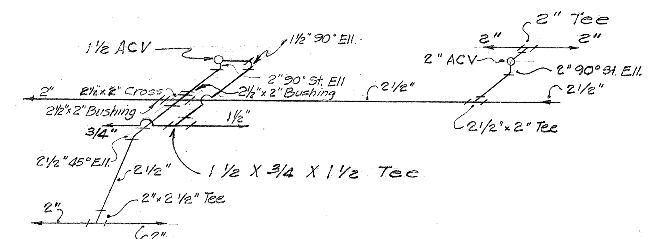
DETAIL 1-D
