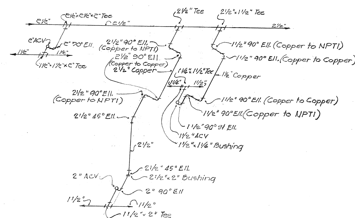
DETAIL 3-M
