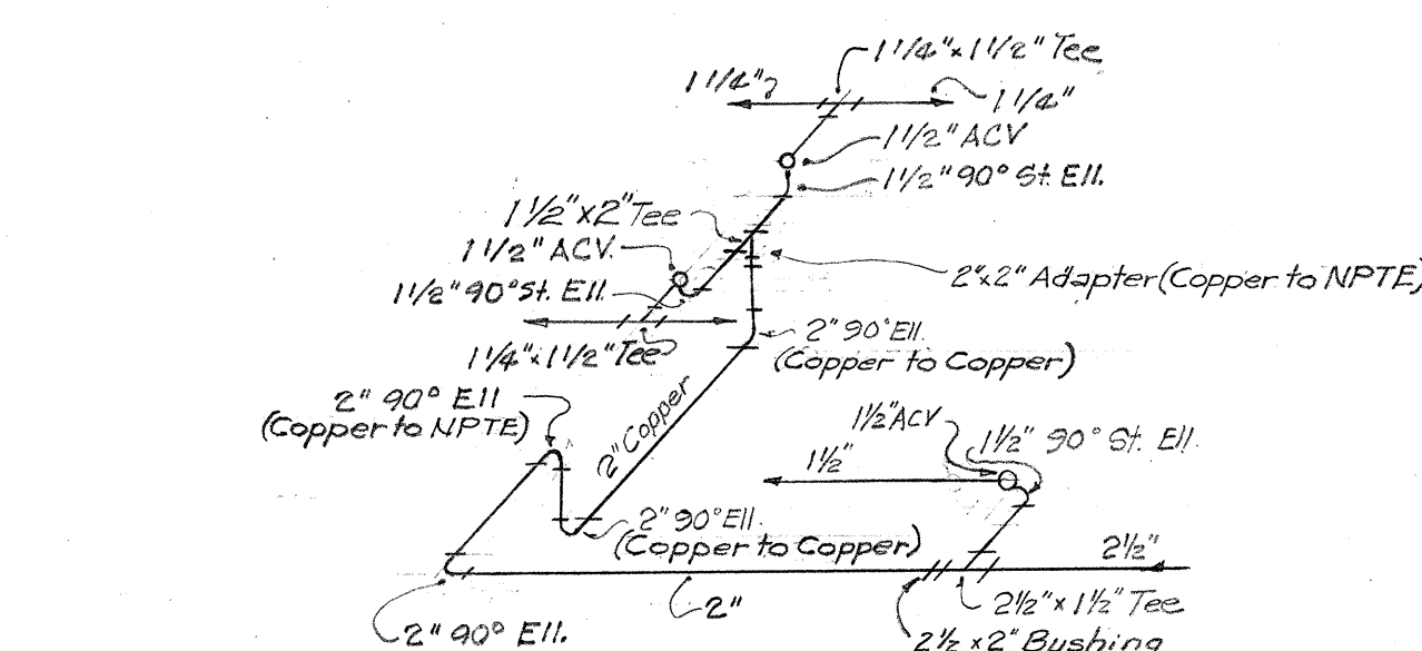
DETAIL 1-F
