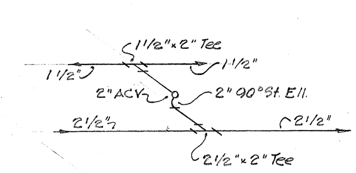
DETAIL 2-E
