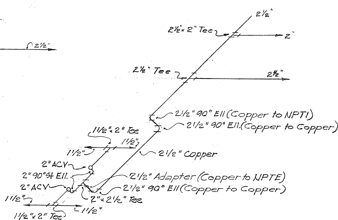
DETAIL 3-F
