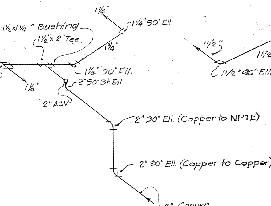
DETAIL 2-B
