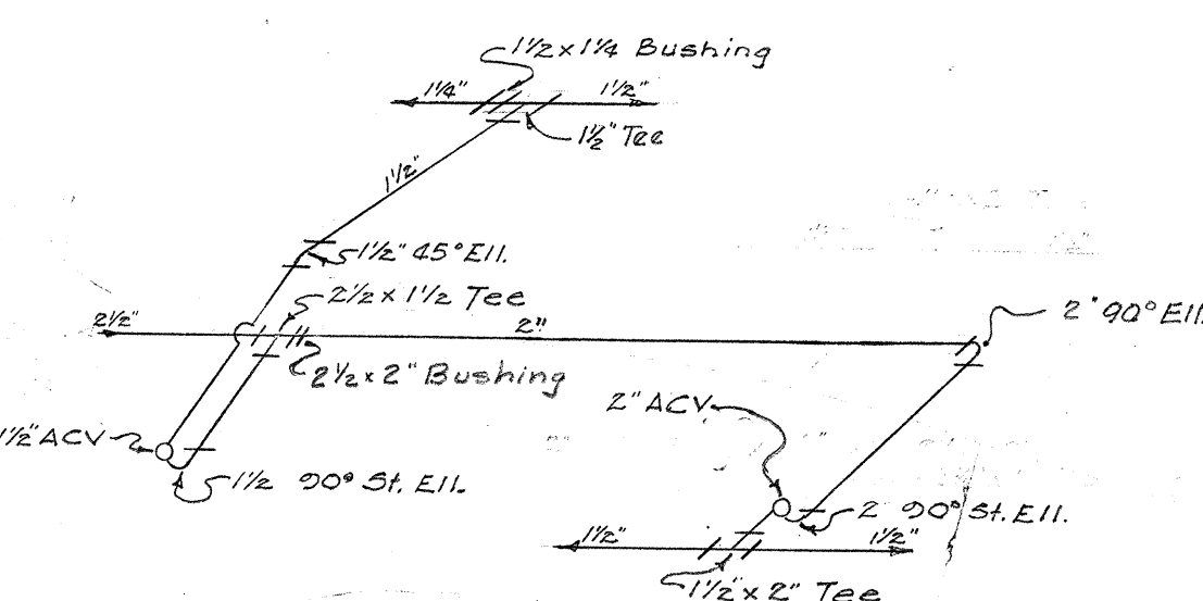
DETAIL 3-K
