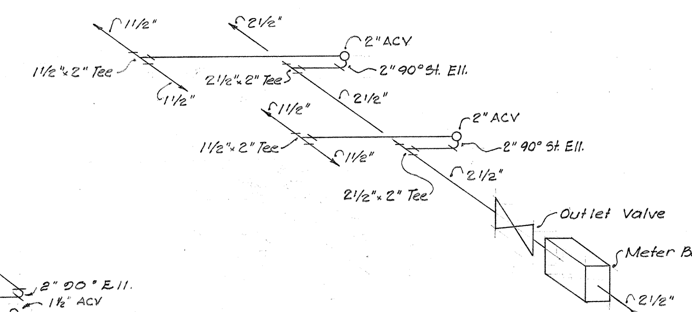
DETAIL 2-K
