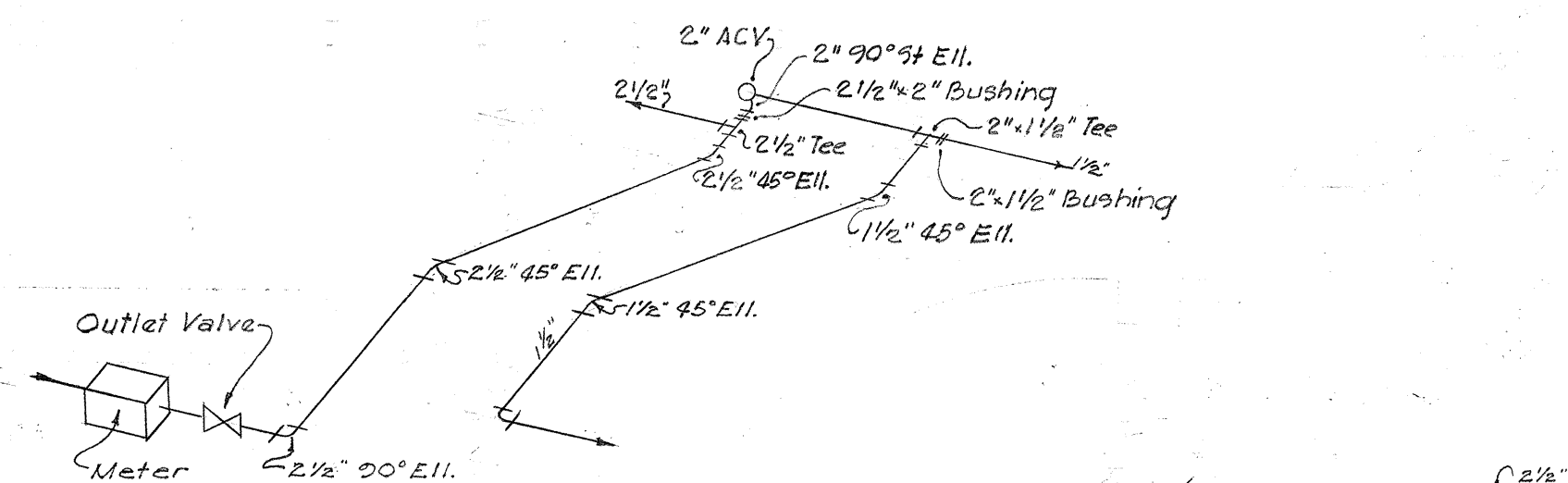
DETAIL 3-D
