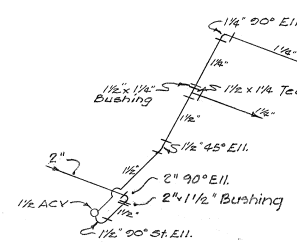
DETAIL 3-L
