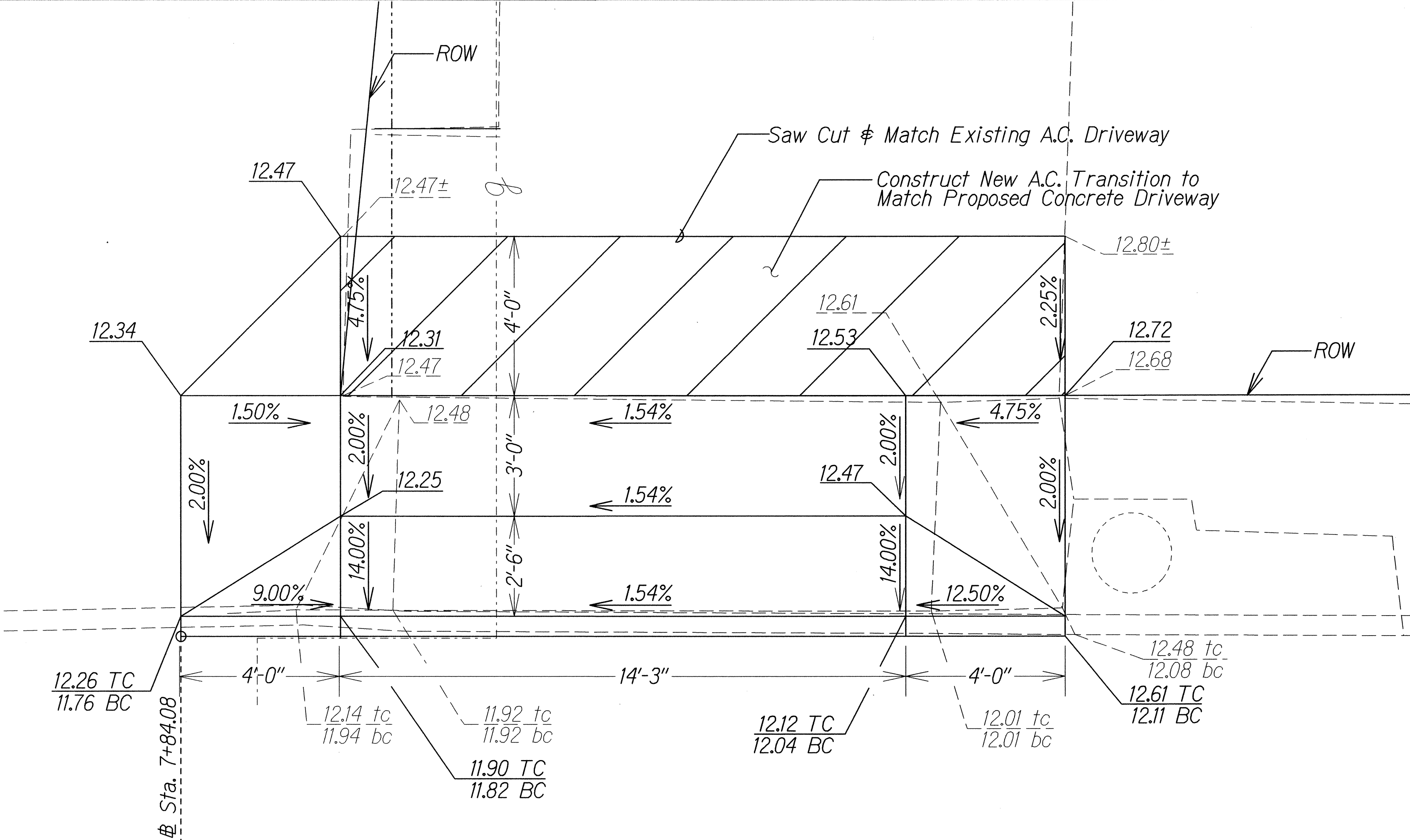
DRIVEWAY @ STA. 7+84± to @ STA. 8+06± LT. Scale: 1/2" = 1'
