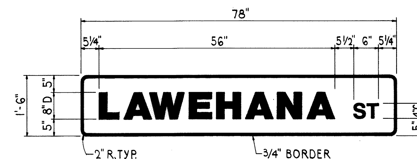
STREET NAME SIGN DETAIL NOT TO SCALE
