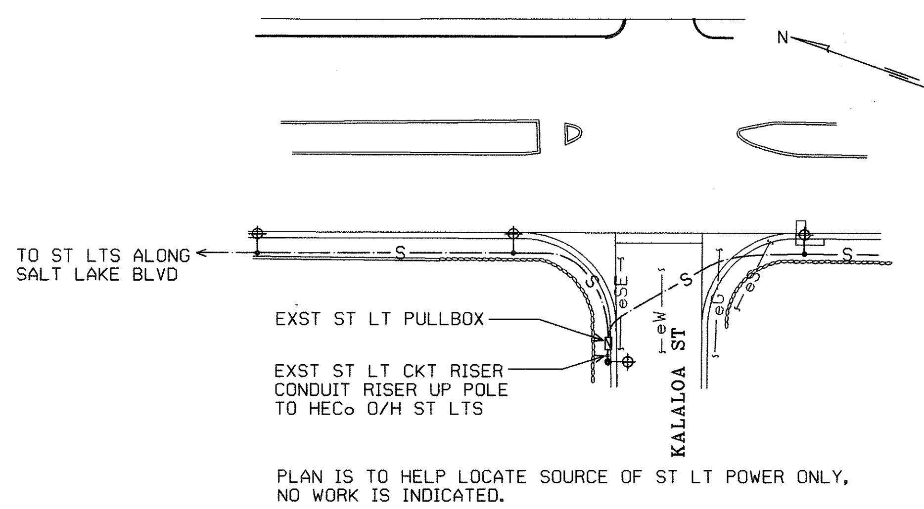
B PARTIAL SITE ELECTRICAL PLAN E-1 SCALE: 1" = 40'-0" 93116-S2
