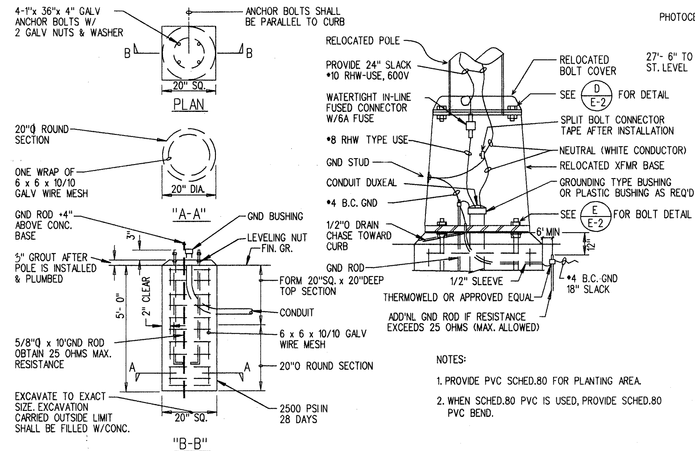
NEW CONCRETE BASE DETAIL
