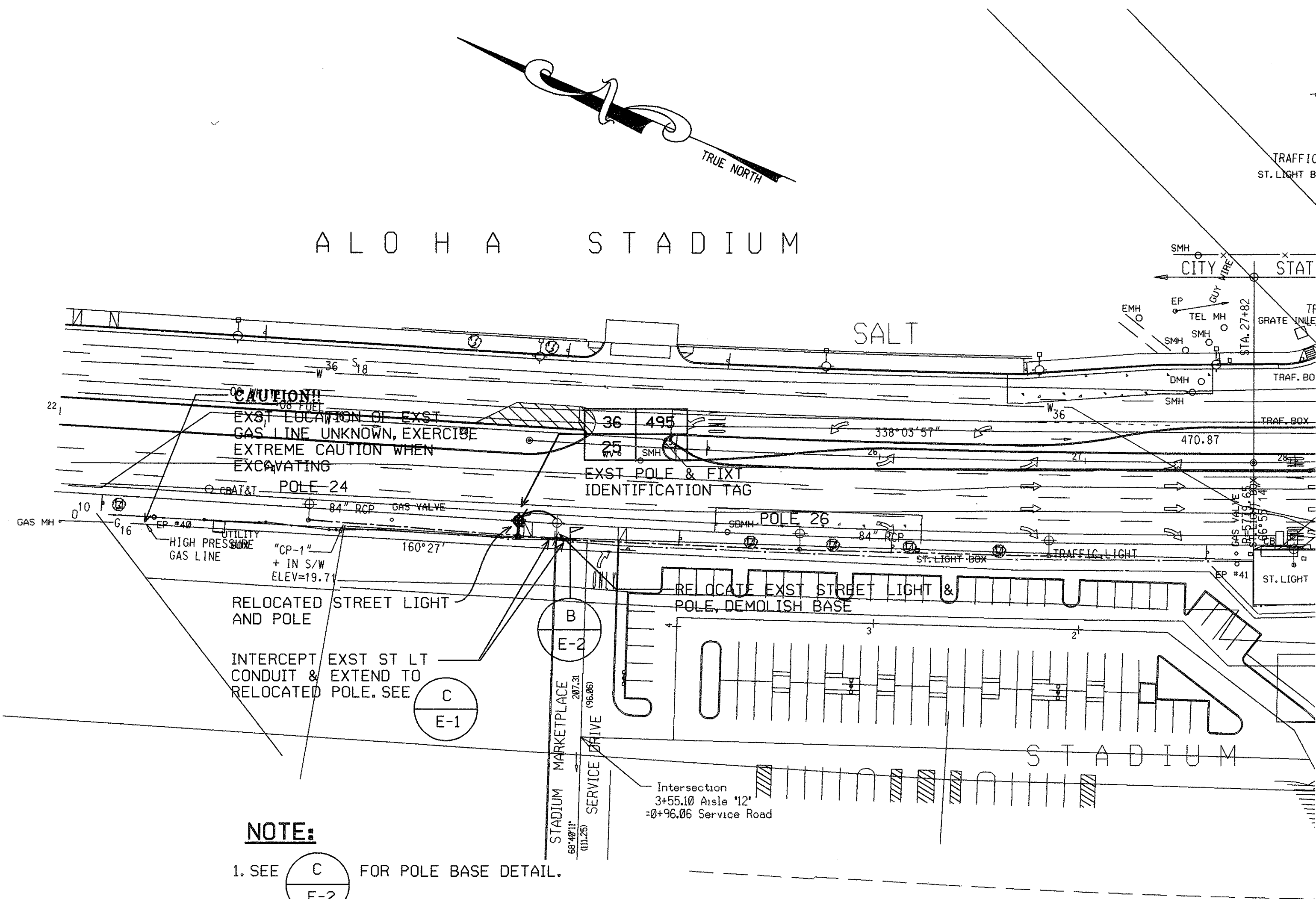
A SITE ELECTRICAL PLAN E-1 SCALE: 1" = 40'-0" 93116-S1
