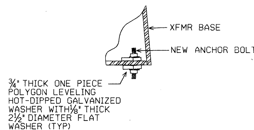
D BOLT DETAIL E-2 93116-B0
