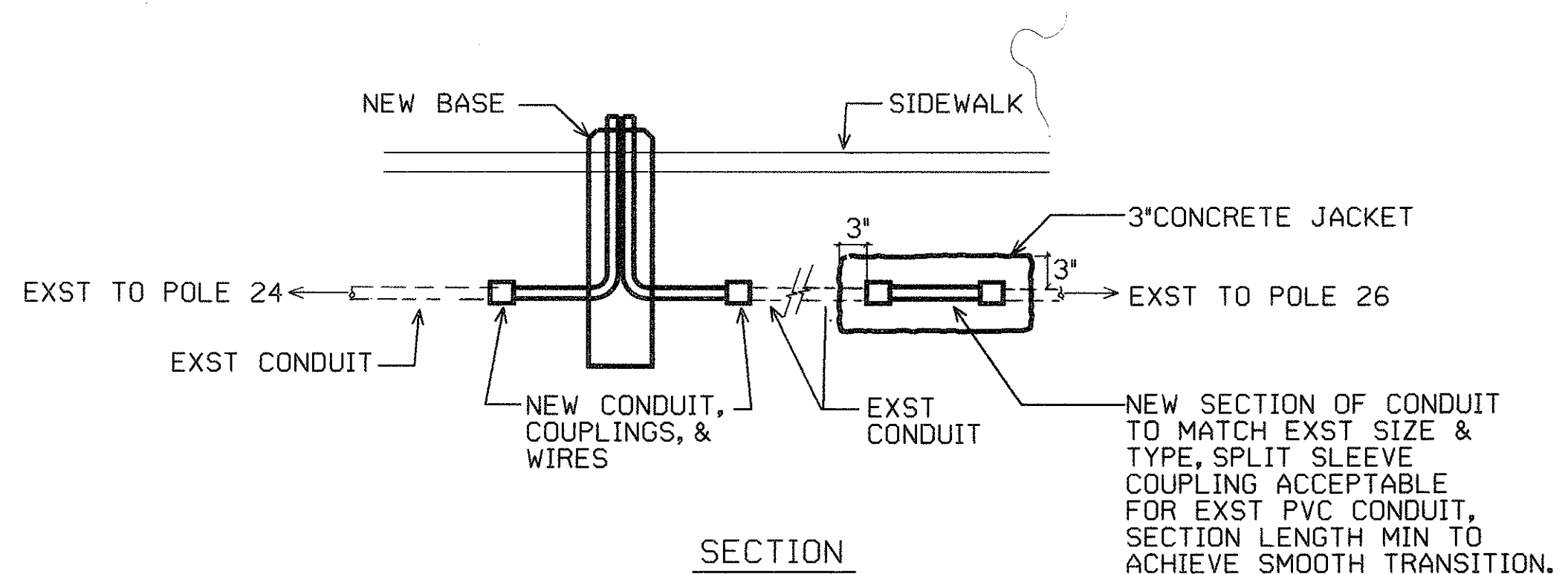
C ST. LT. DUCT DETAIL E-1 NO SCALE 93116SD
