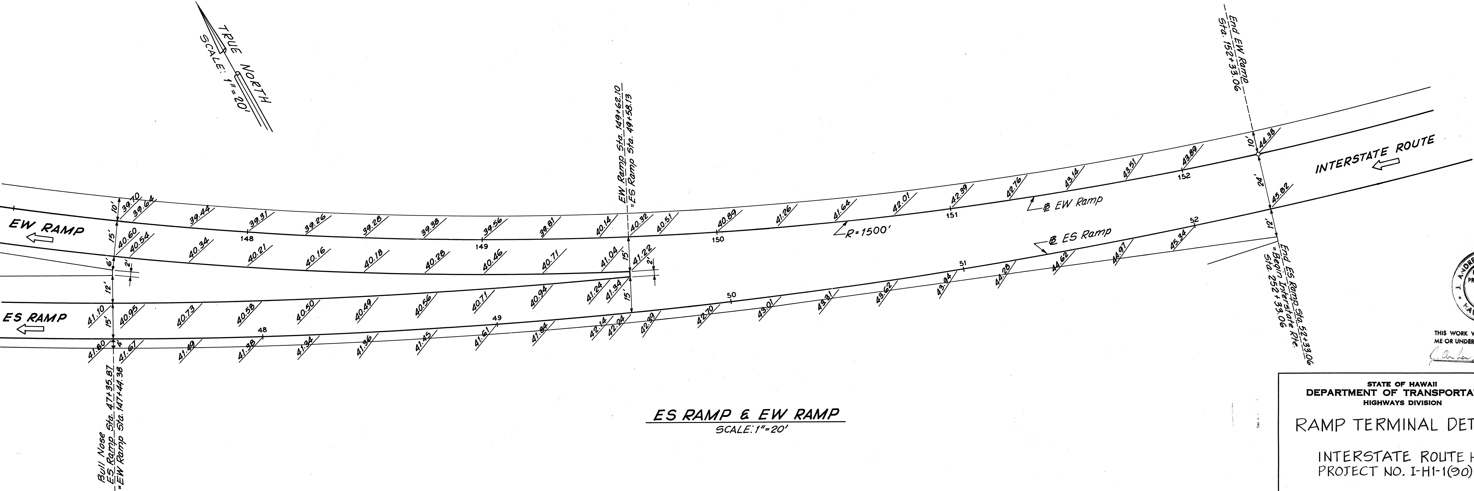
RAMP P & INTERSTATE ROUTE SCALE: 1"=20'
