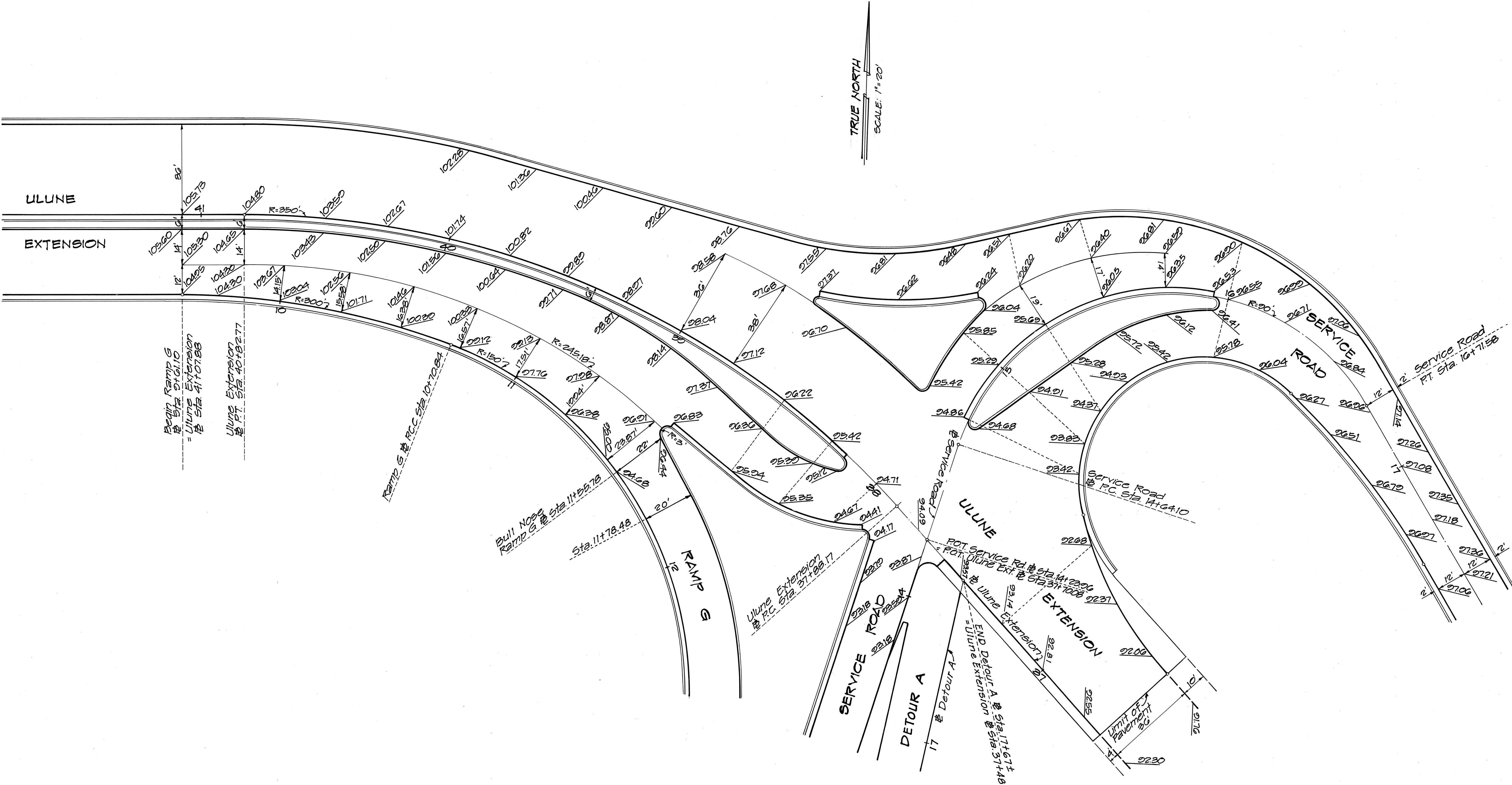
ULUNE EXTENSION, RAMP G & SERVICE ROAD Scale: 1"=20'
