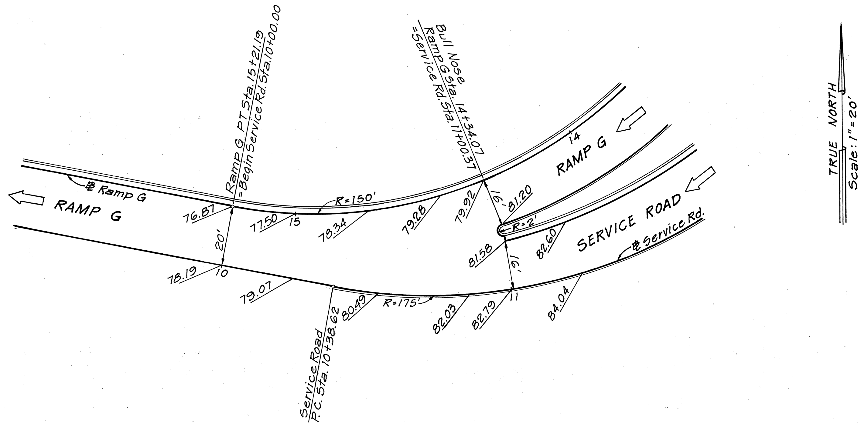
RAMP G & SERVICE ROAD SCALE: 1" = 20'
