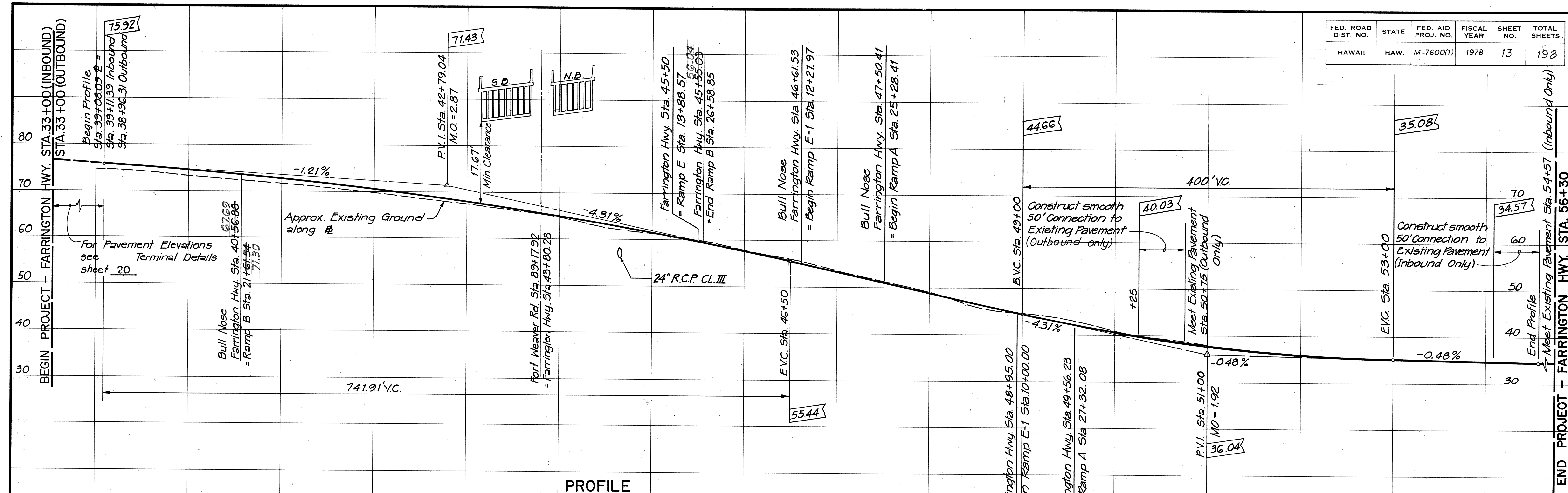
PROFILE SCALE: HOR. 1" = 50' VERT. 1" = 10'
