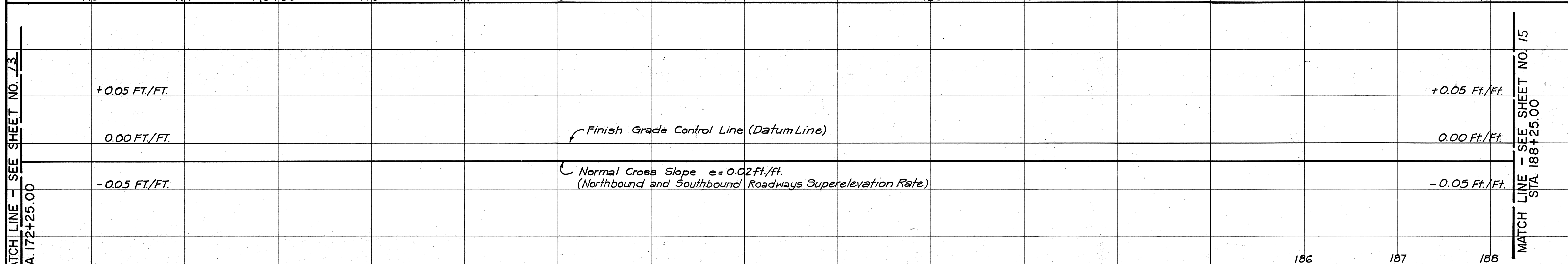
SUPERELEVATION DIAGRAM SCALE: HOR. 1" = 50' VERT. 1" = 0.05 FT./FT. For Notes See Sheet No. 13
