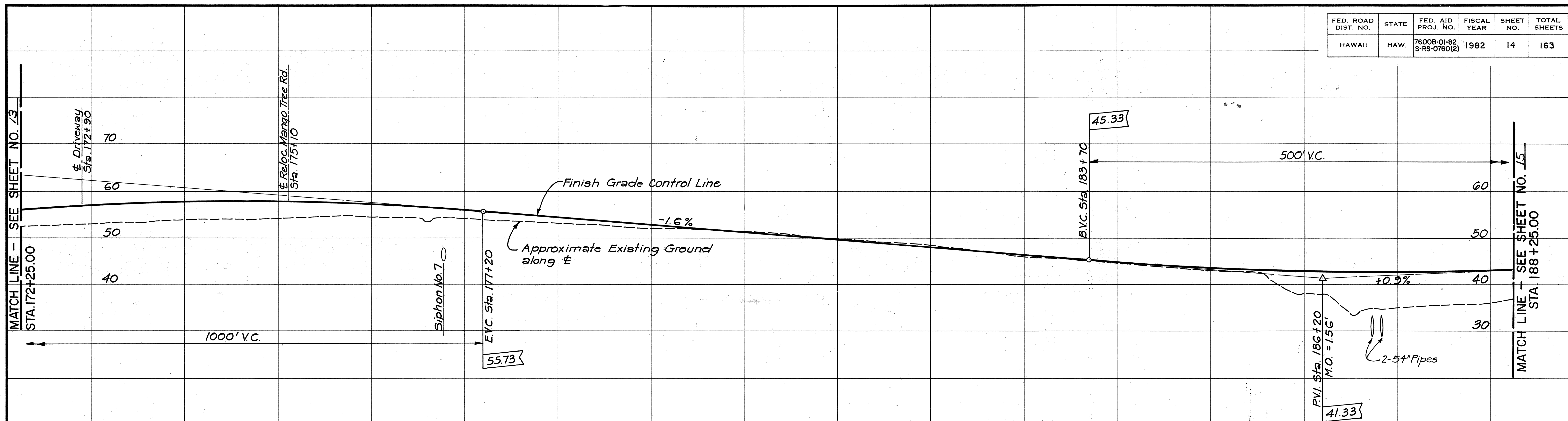
PROFILE SCALE: HOR. 1" = 50' VERT. 1" = 10' For Notes See Sheet No. 13
