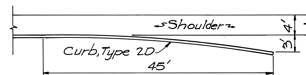
TYPICAL END TREATMENT FOR CURB, TYPE 2D N.T.S.
