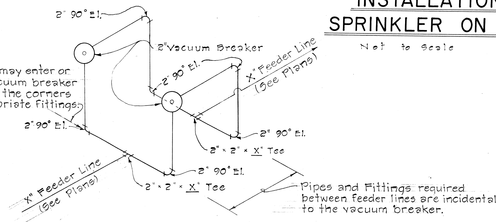
DOUBLE - 2" VACUUM BREAKER Not to Scale
