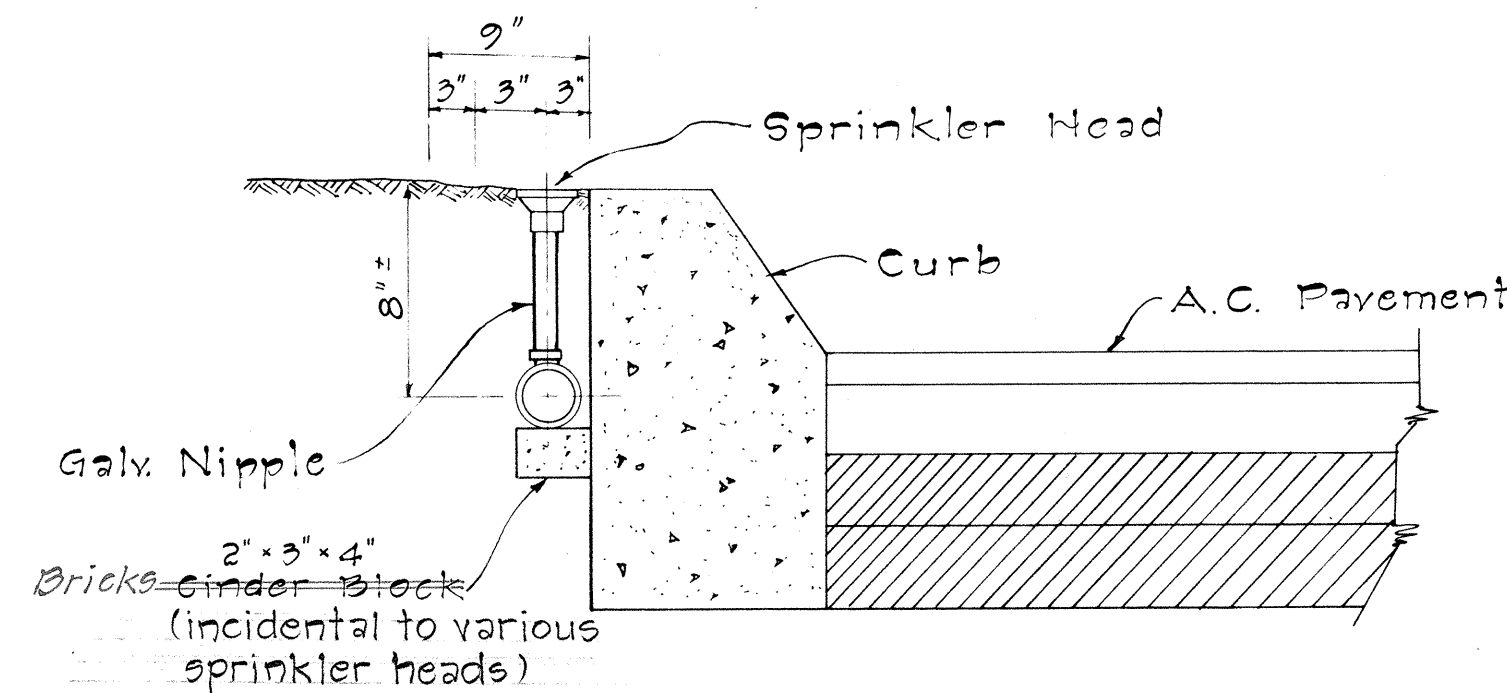
TYPICAL DETAIL OF SPRINKLER HEAD AT CONC. CURB Not to Scale
