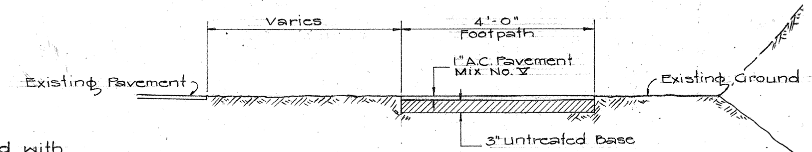
TYPICAL SECTION OF ASPHALT FOOTPATH
