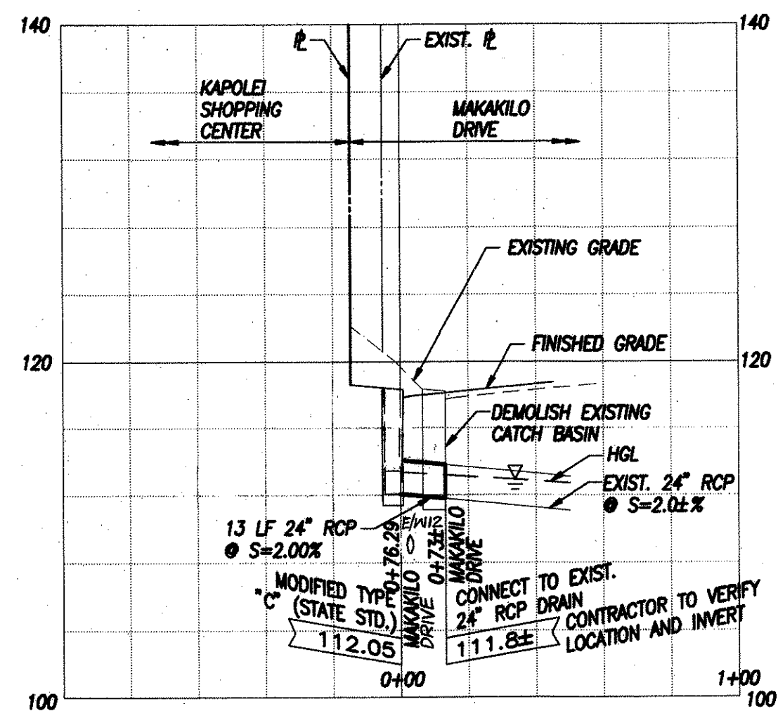
PROFILE - DRAINLINE EXTENSION AT 0+76± MAKAKILO DRIVE
