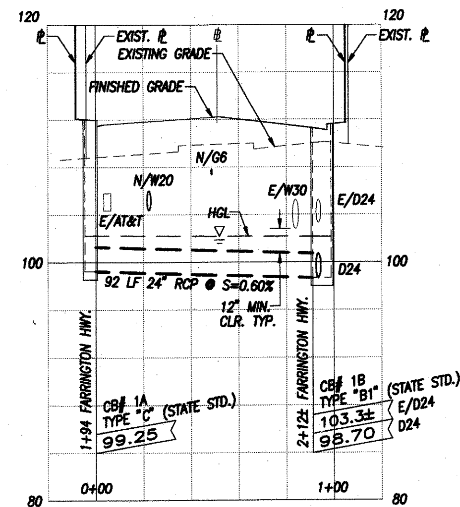
PROFILE - DRAINLINE FROM CB# 1A TO CB# 1B
