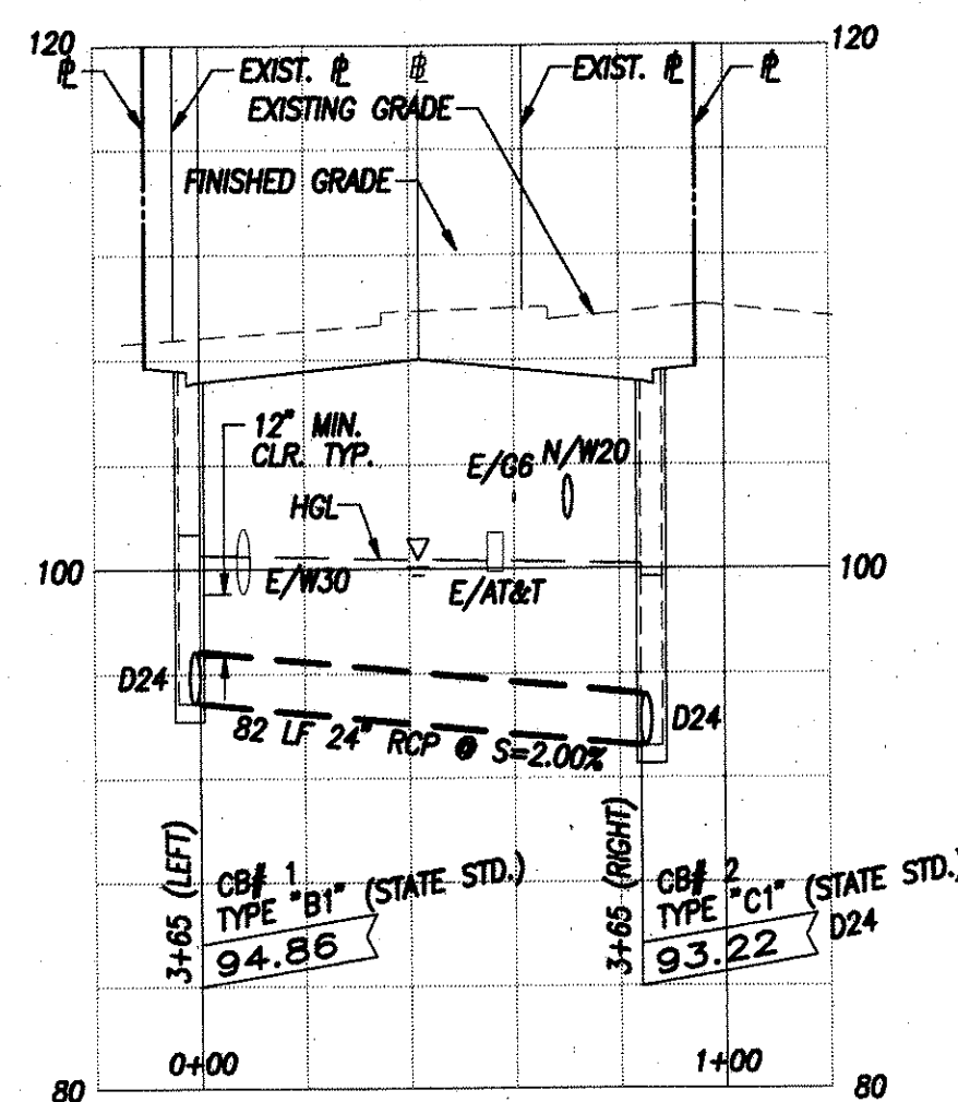
PROFILE - DRAINLINE FROM CB# 1 TO CB# 2
