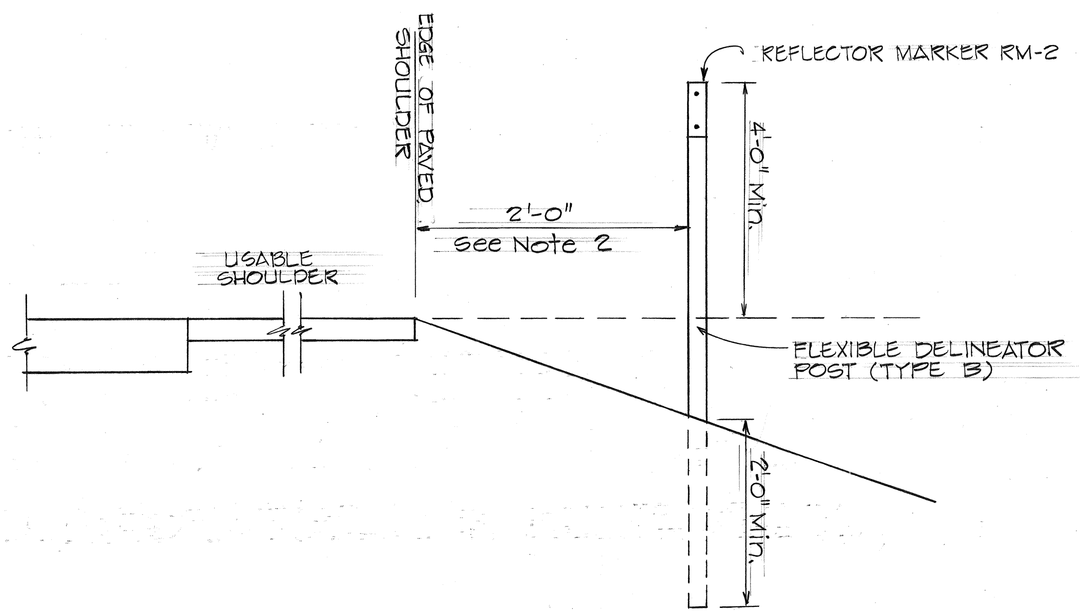
REFLECTOR MARKER MOUNTING DETAIL N.T.S.
