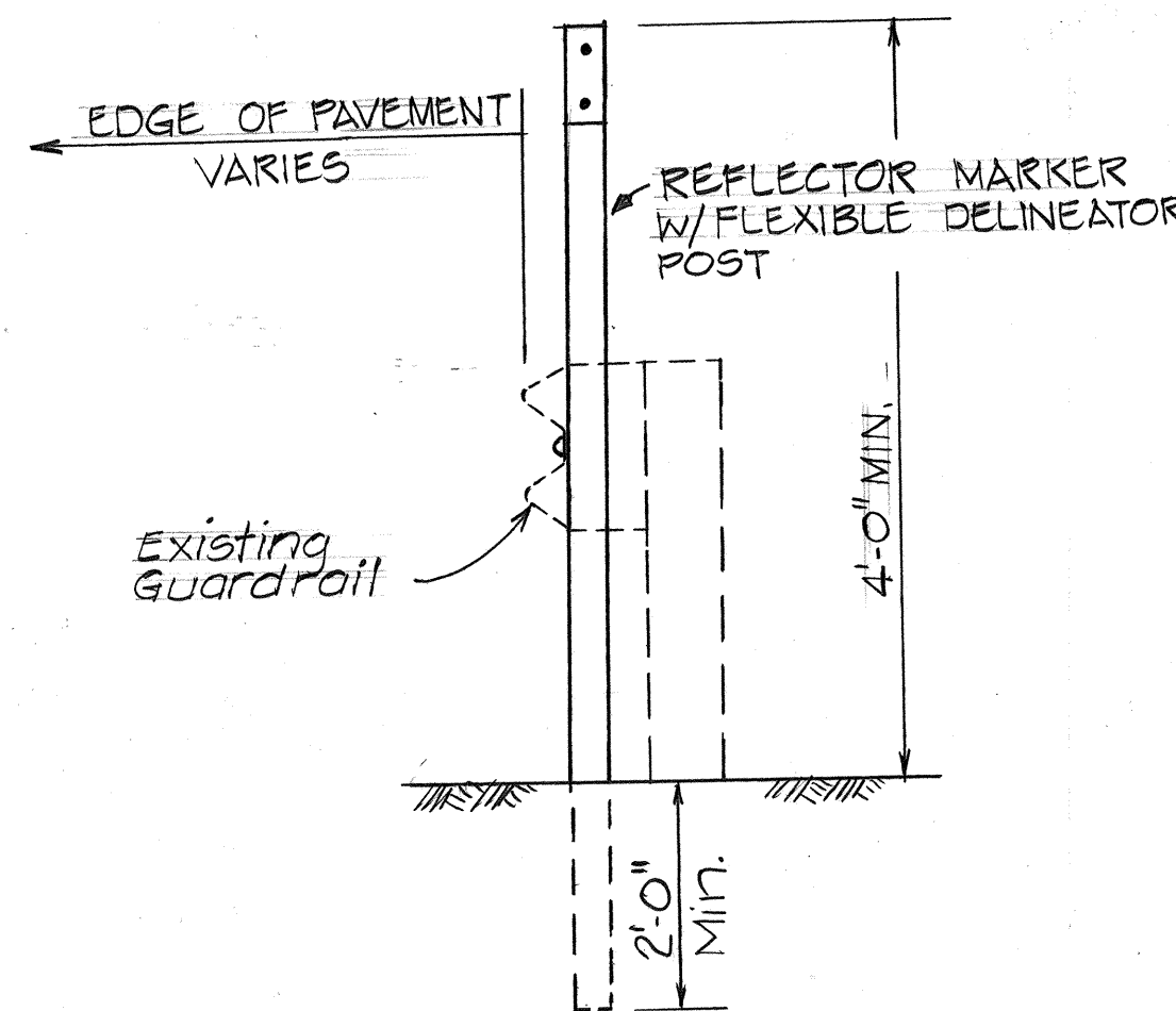
TYPICAL DETAIL REFLECTOR MARKER INSTALLATION BEHIND GUARDRAIL N.T.S.
