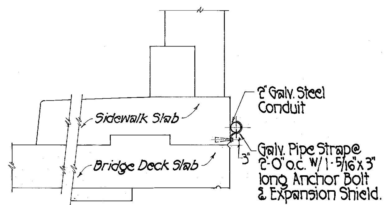
2" GALV. STEEL CONDUIT ATTACH. TO BRIDGE Scale: 1"=1'-0"
