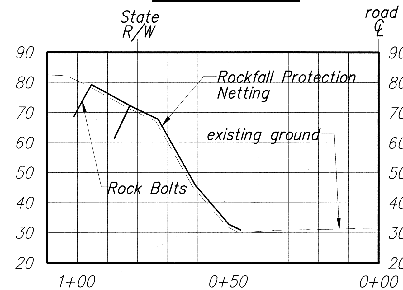
Station 48+75
