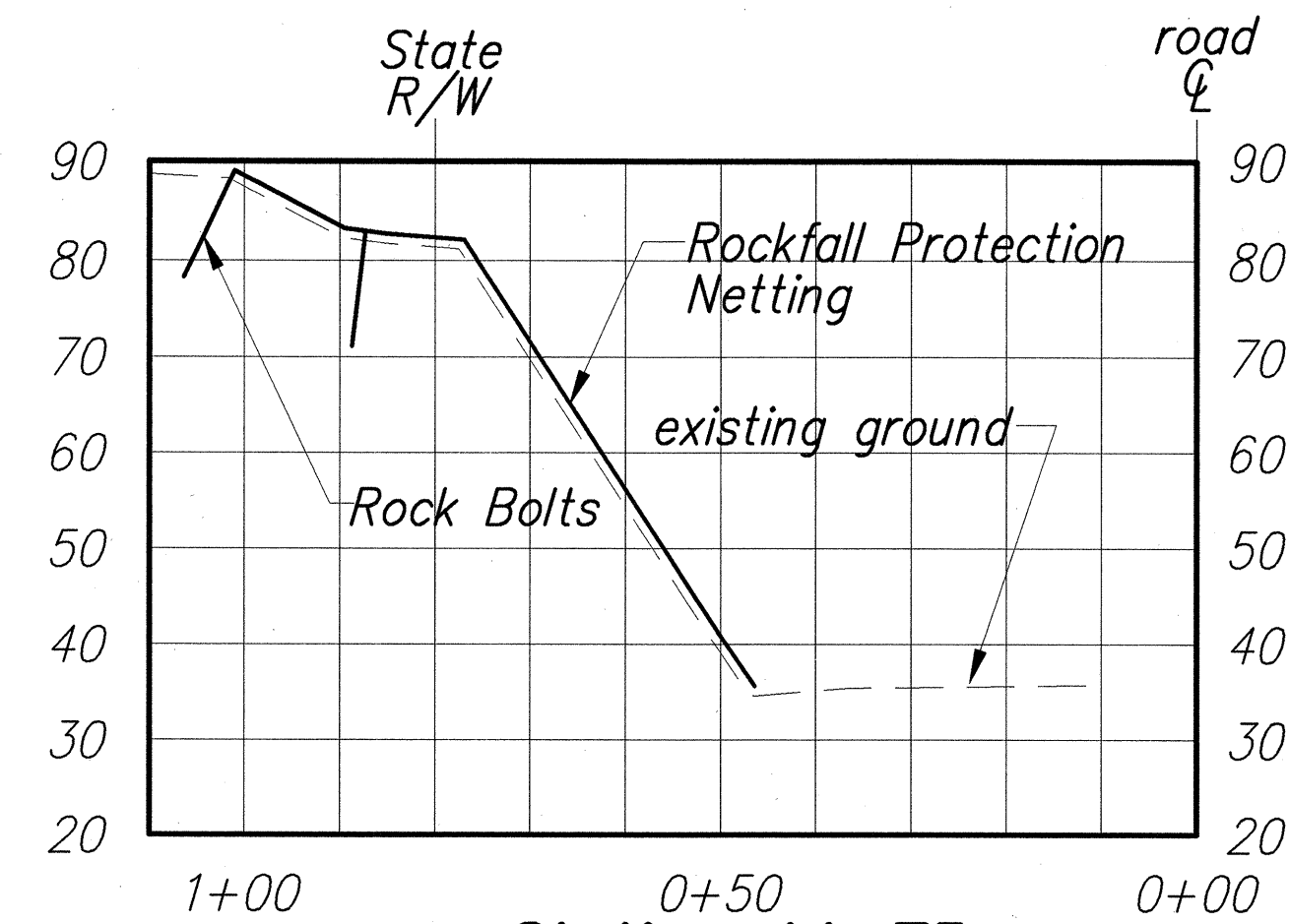
Station 44+75
