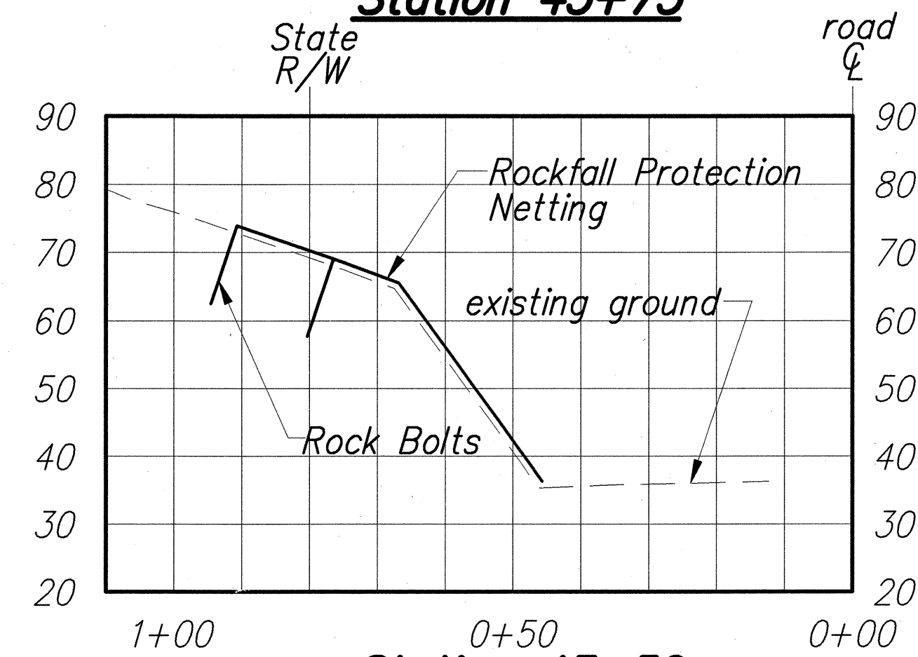
Station 43+50
