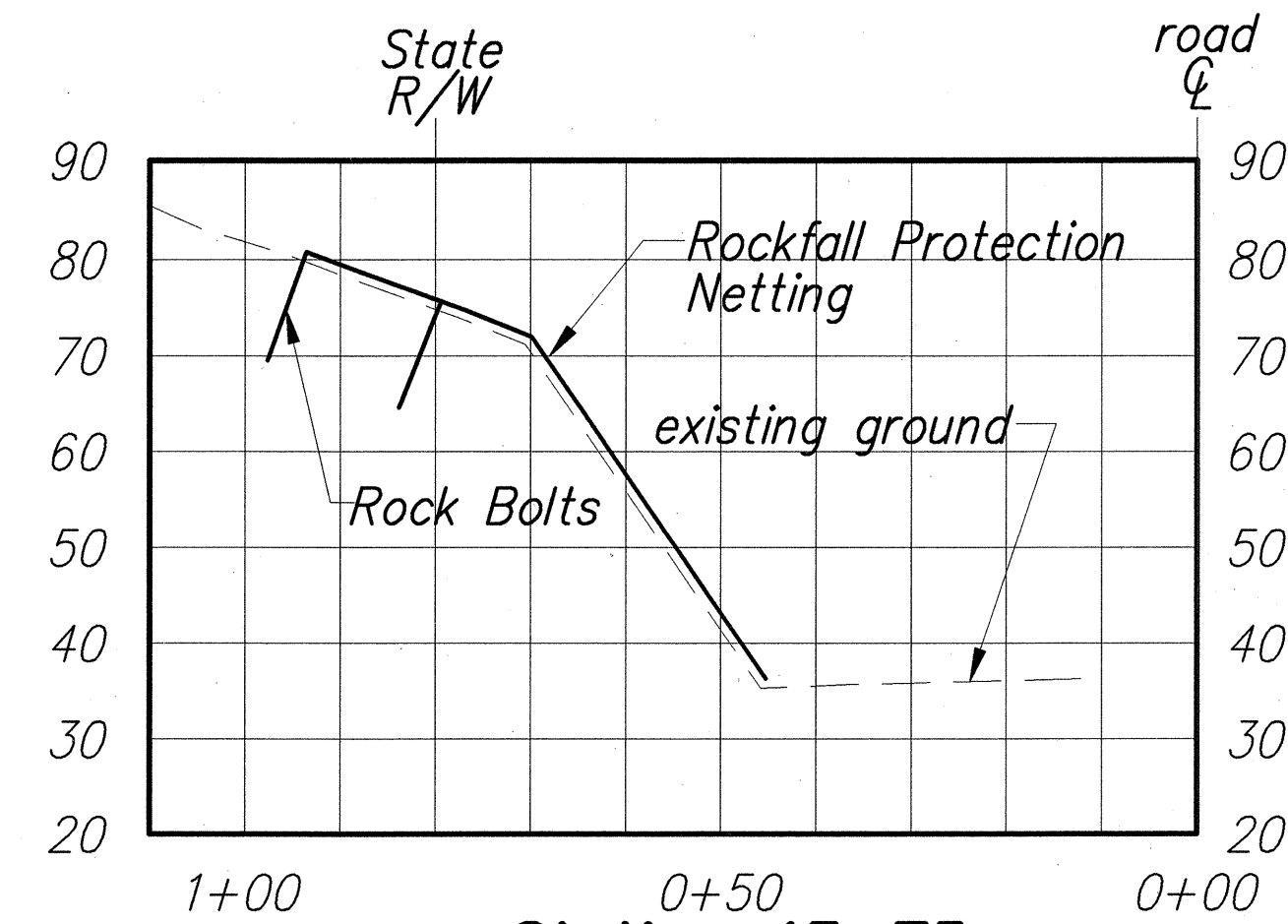
Station 43+75
