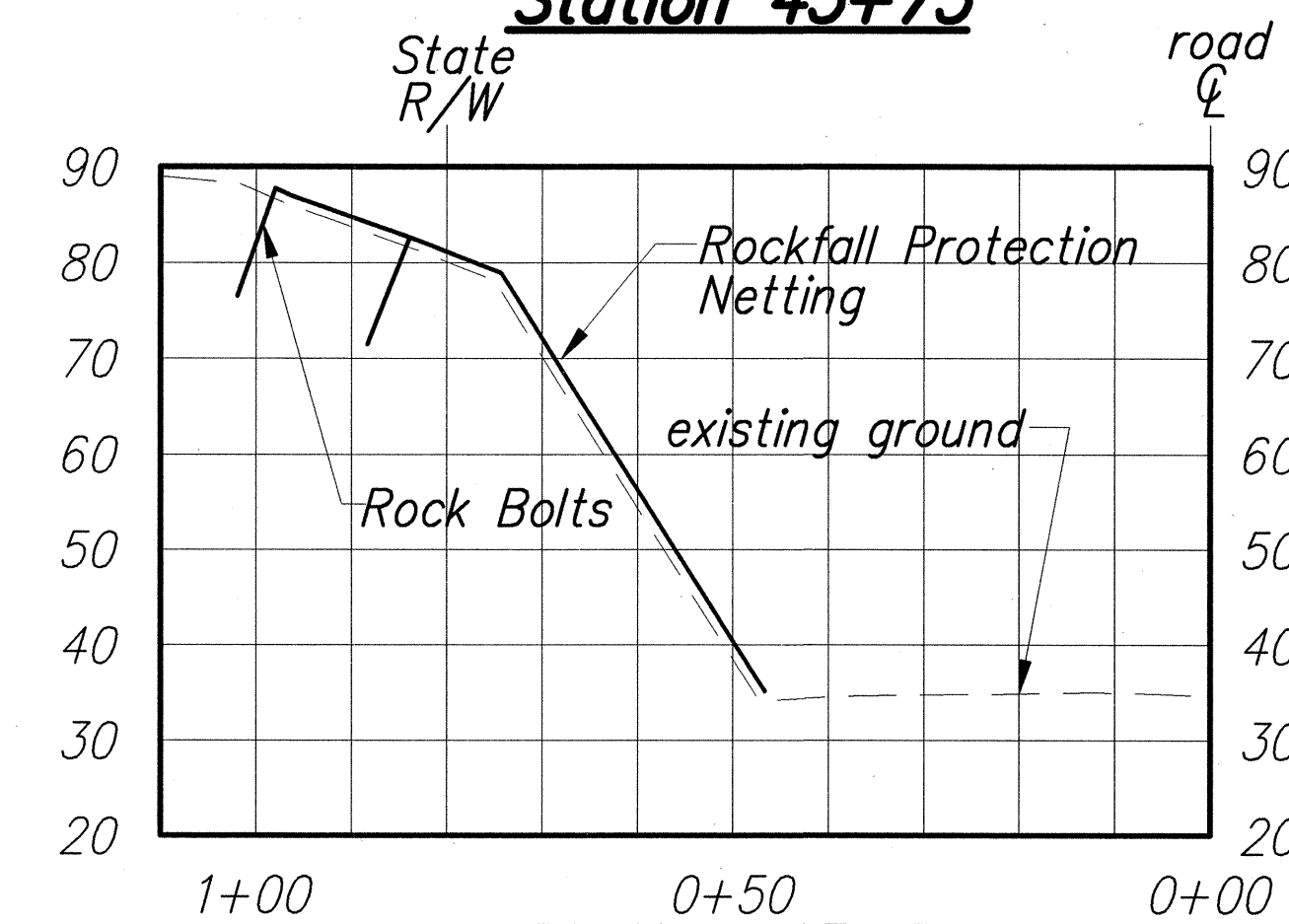
Station 45+50
