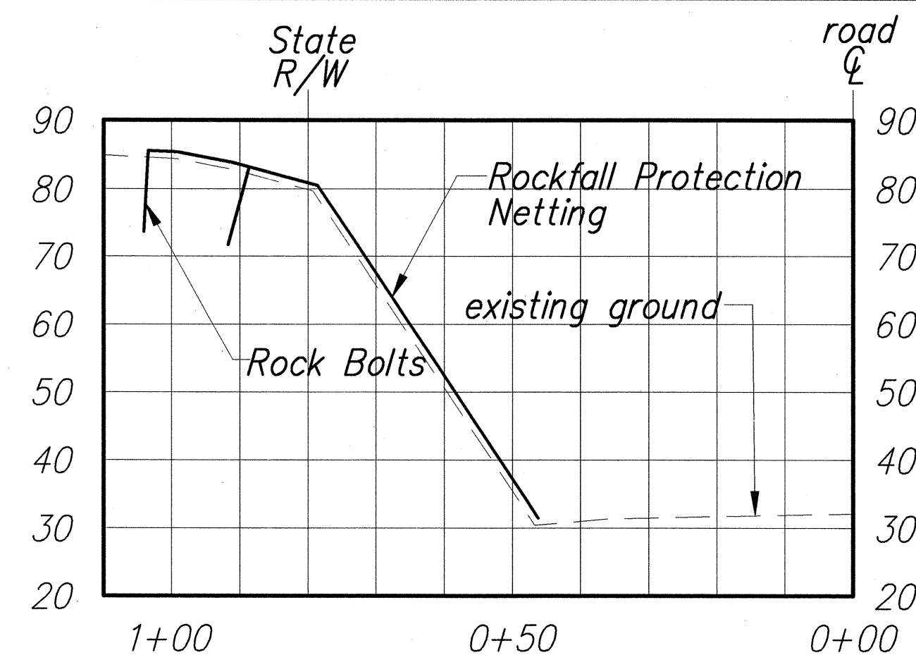
Station 48+25
