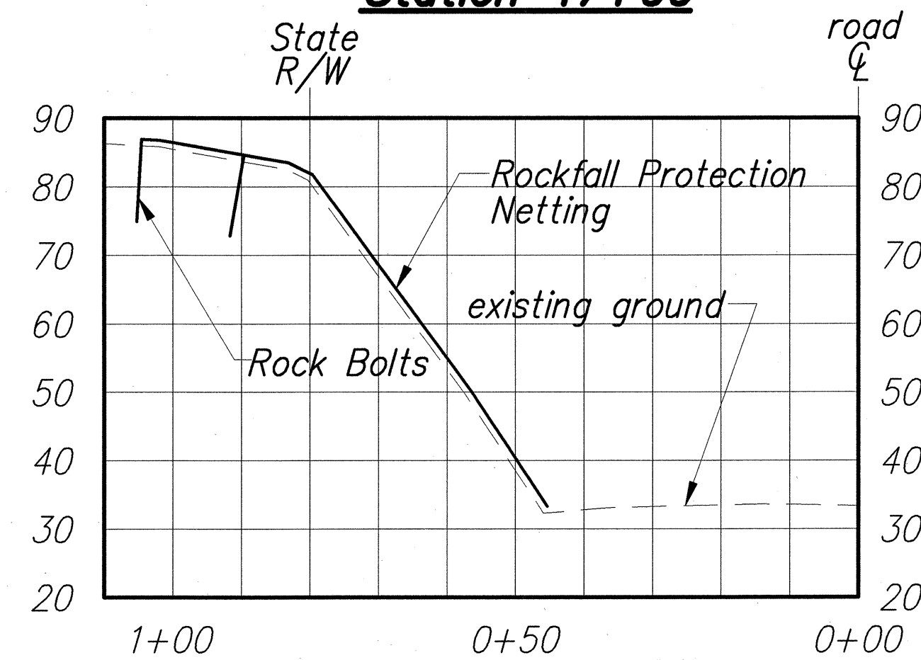
Station 46+75
