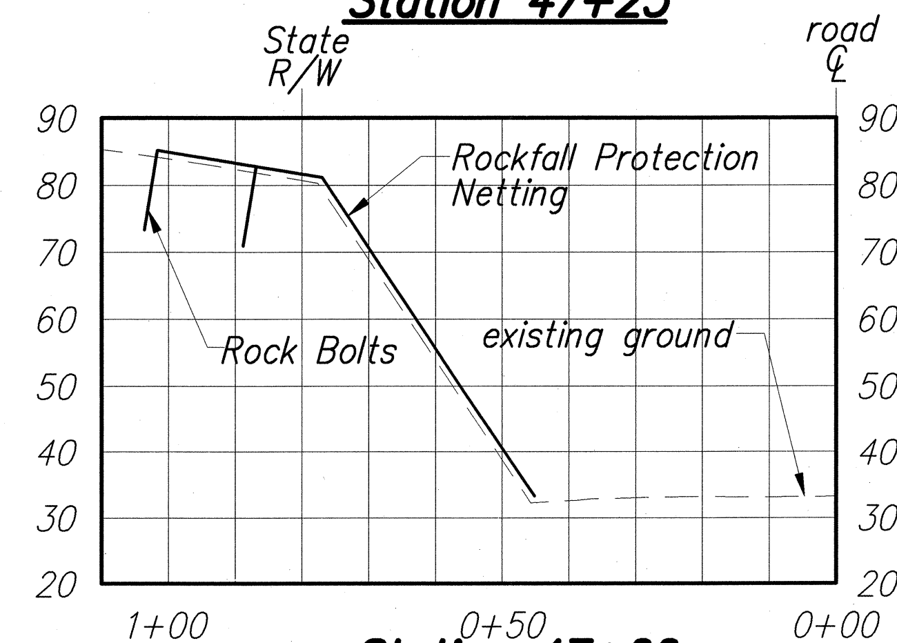
Station 47+00
