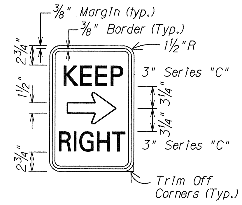
SIGN R4-7a(R) 12"x18" Not to Scale
