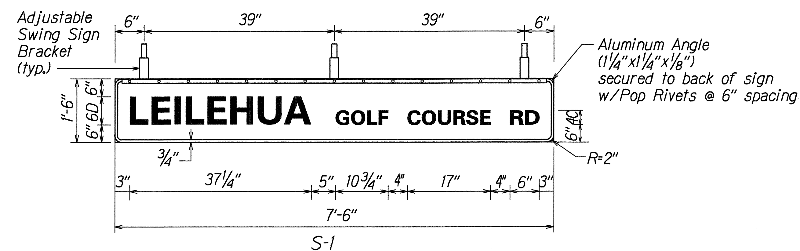
(Rear View) PANEL & SWING BRACKET LAYOUT FOR STREET NAME SIGN
