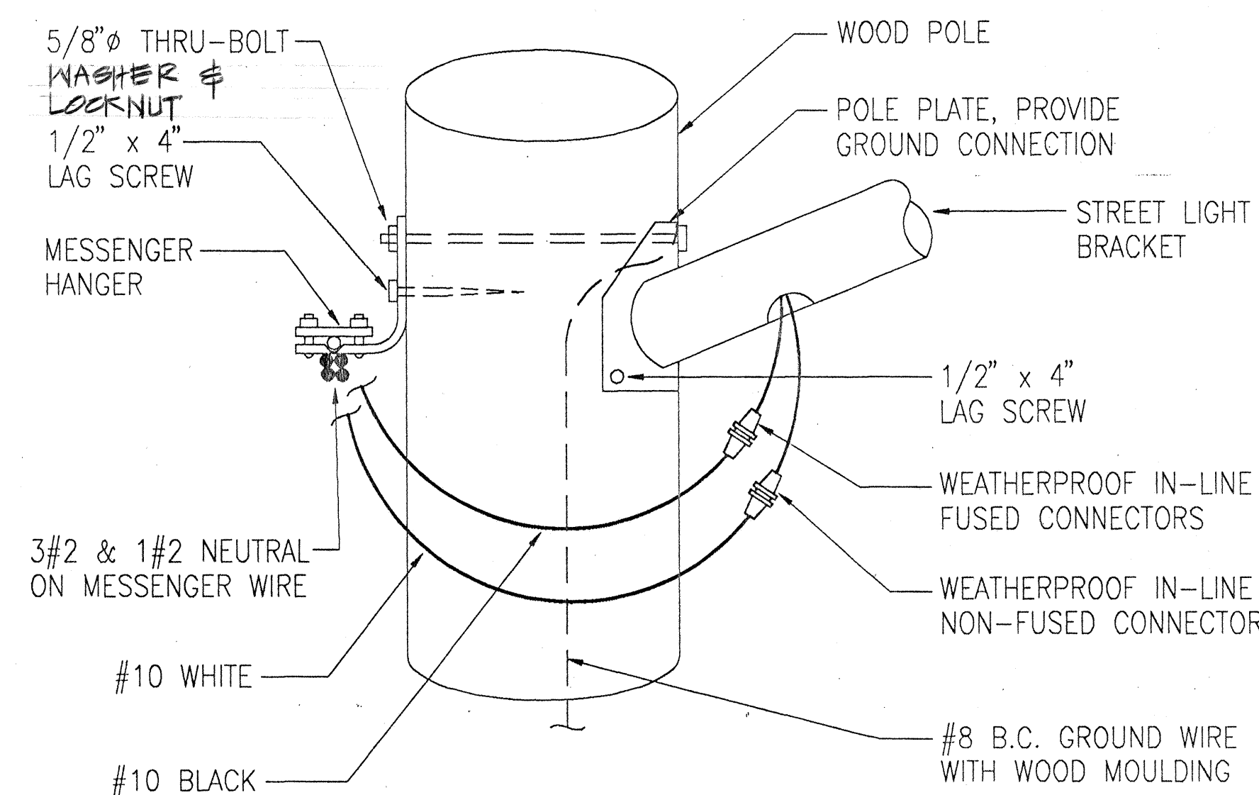
3 DETAIL NOT TO SCALE CAD: 4010-E4
